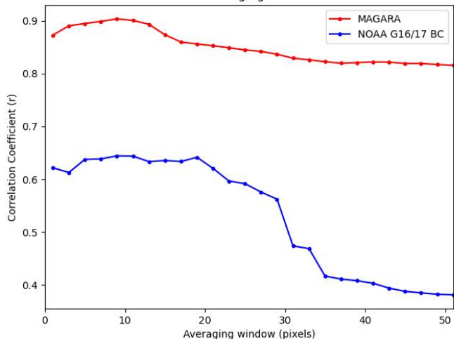
225 Figure S5) Same as Figure S2, but without requiring a good QA retrieval directly over the AERONET station for either MAGARA or NOAA.
