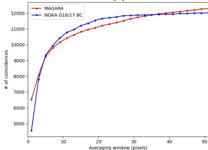
225 Figure S5) Same as Figure S2, but without requiring a good QA retrieval directly over the AERONET station for either MAGARA or NOAA.
