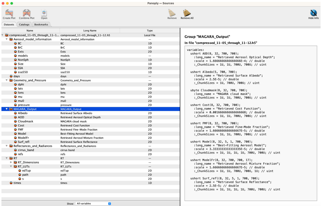
160 Figure S1) Example MAGARA output file as viewed in Panoply. This output file represents the output for the Camp Fire.
