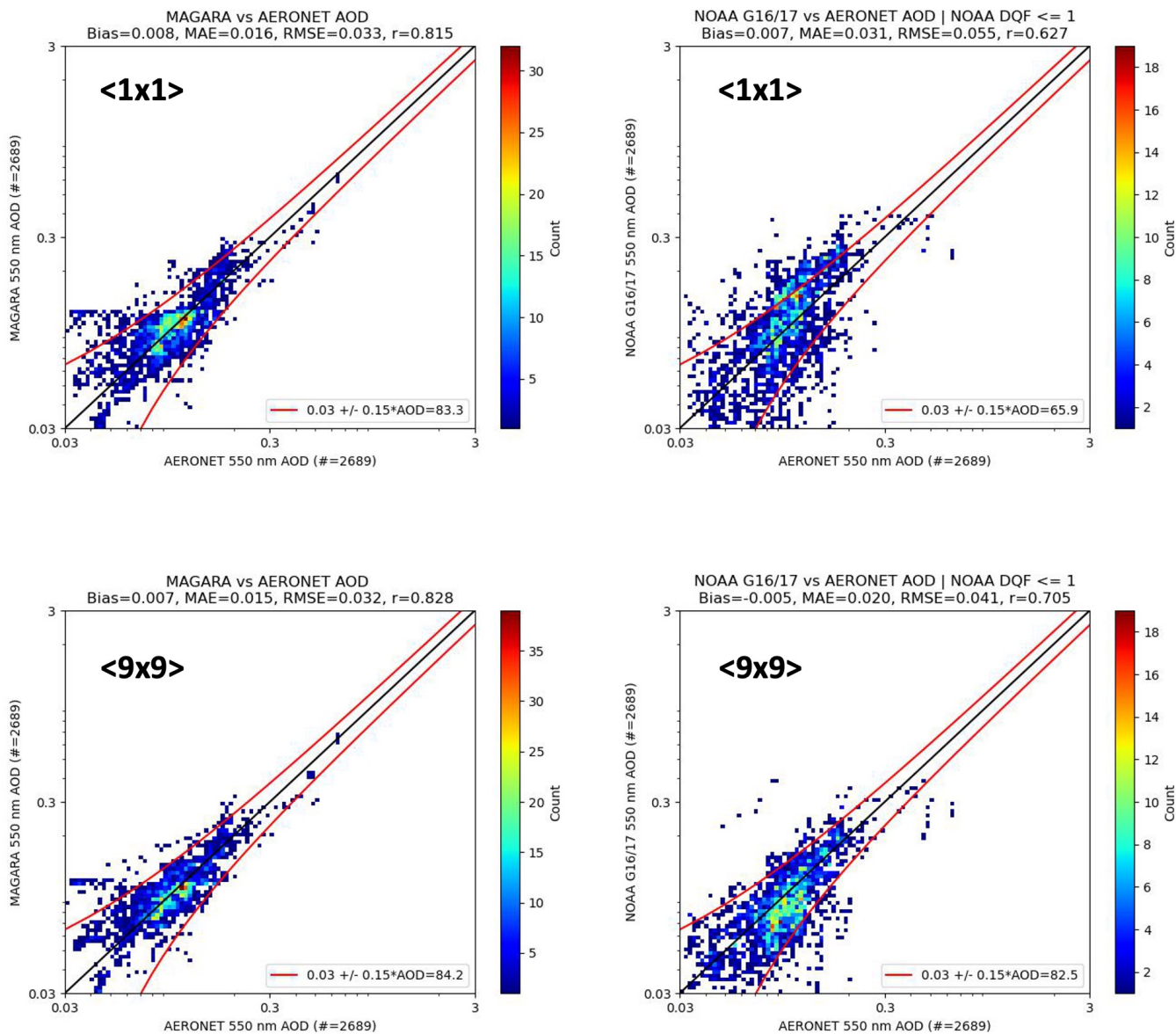
205 Figure S3) 2-D histograms of MAGARA and NOAA bias corrected 550 nm AOD retrievals vs AERONET 550 nm AOD. Upper left panel represents the MAGARA vs AERONET 550 nm AOD 2-D histogram using only the MAGARA retrieval centered on the AERONET site. Upper right panel represents the NOAA G16/17 bias corrected vs AERONET 550 nm AOD 2-D histogram using only the NOAA retrieval centered on the AERONET site. Bottom rows represent the same as the top row, but with 9 x 9 210 pixel spatial averaging for the satellite retrievals. A standard \pm (0.03 + 0.15 * AOD) uncertainty envelope is provided for reference, with the percent meeting that threshold indicated. Statistics for each panel are presented in the title.
