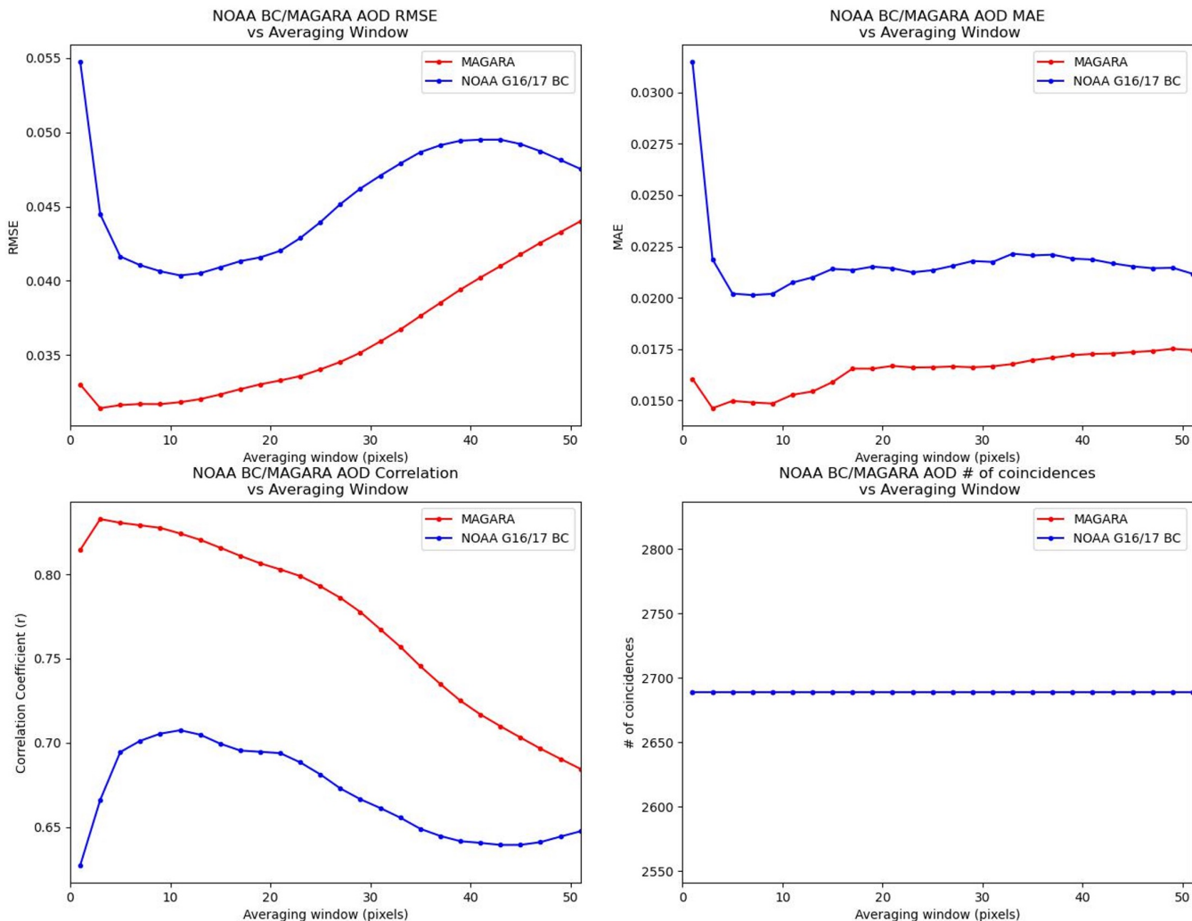
200 Figure S2) MAGARA and NOAA bias corrected error statistics as a function of averaging distance (box average in the x-and-y directions). Root-mean squared error (RMSE) is presented in the upper left, median-absolute error (MAE) is presented in the upper right, Pearson linear correlation coefficient ( r ) is presented in the lower left, and the number of coincidences is presented in the lower right panel.
