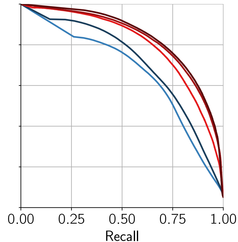
(c) MRMS (2020)
