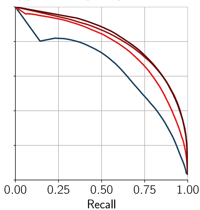
(e) MRMS (2022)
