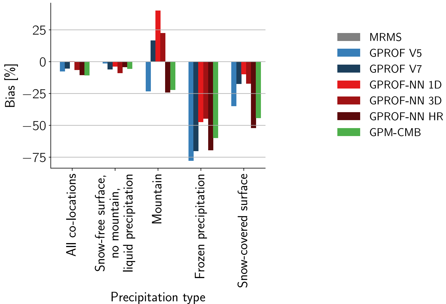
(b) Relative biases
