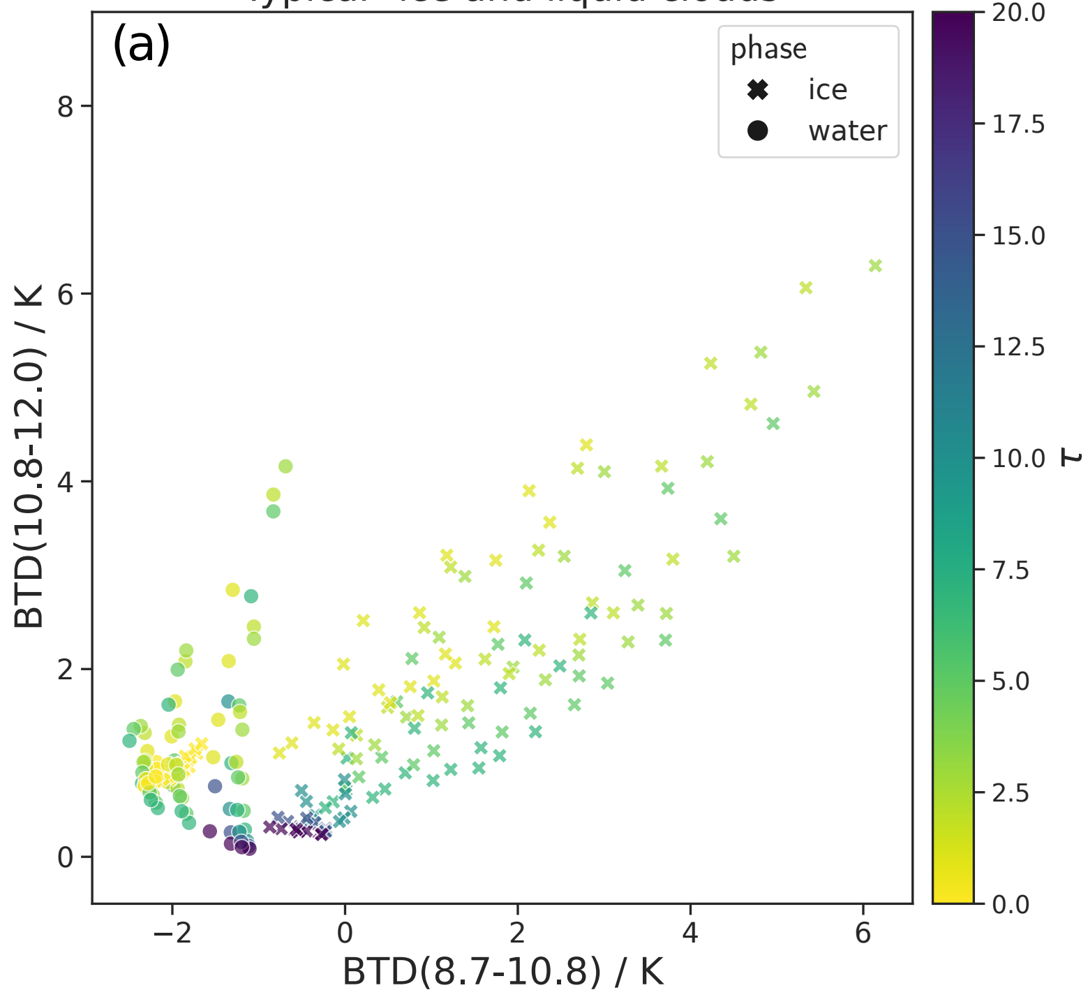
"Typical" ice and liquid clouds
