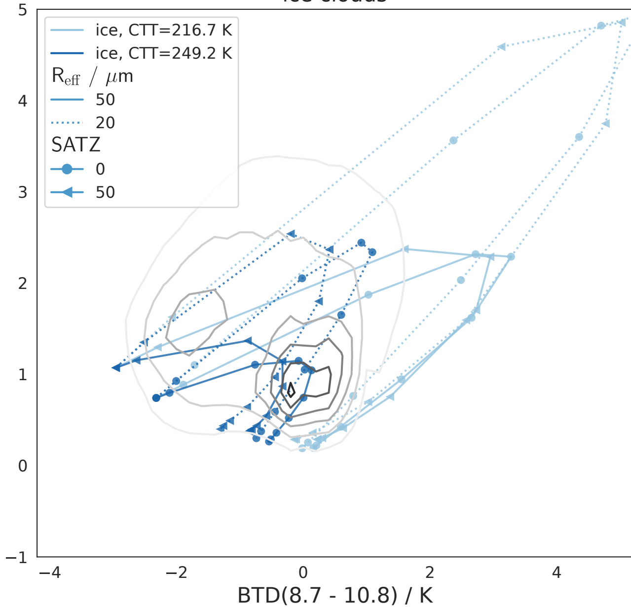
ice clouds
