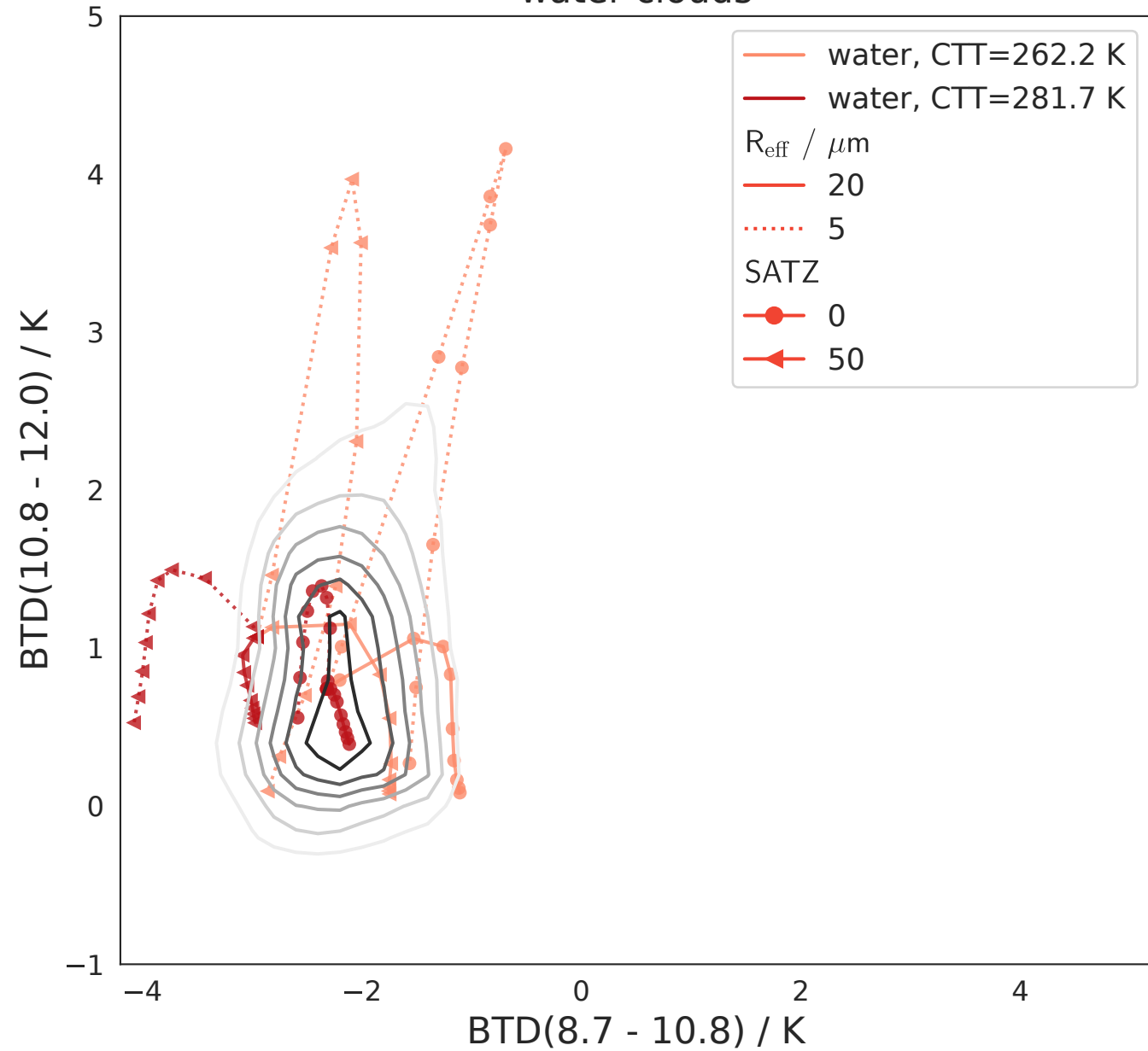
water clouds
