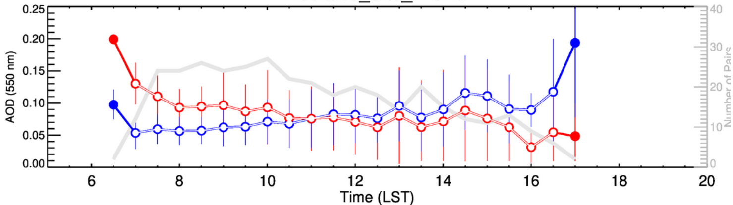
Adelaide_Site_7-OND
