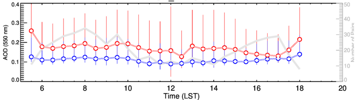
NEON_MLBS-OND
