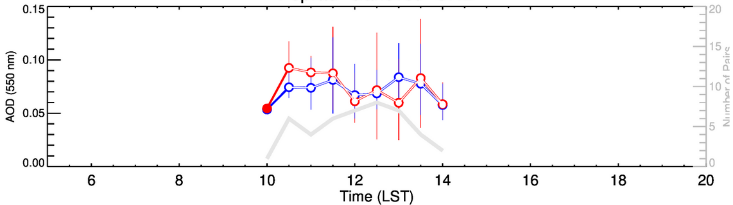
Poprad-Ganovce-OND
