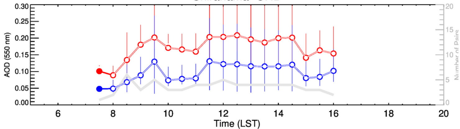
Shirahama-JFM
