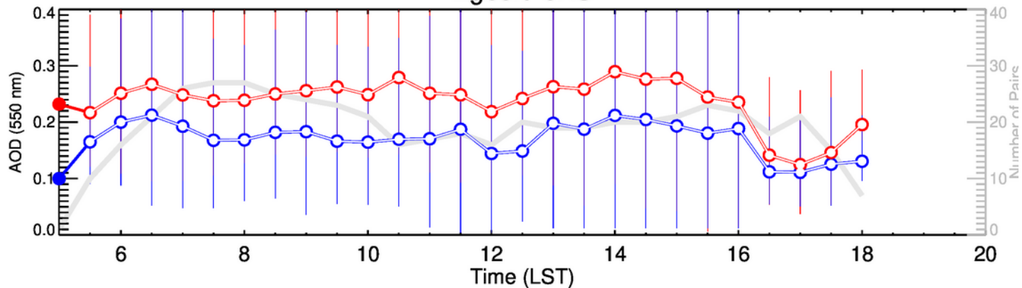
Egbert-OND
