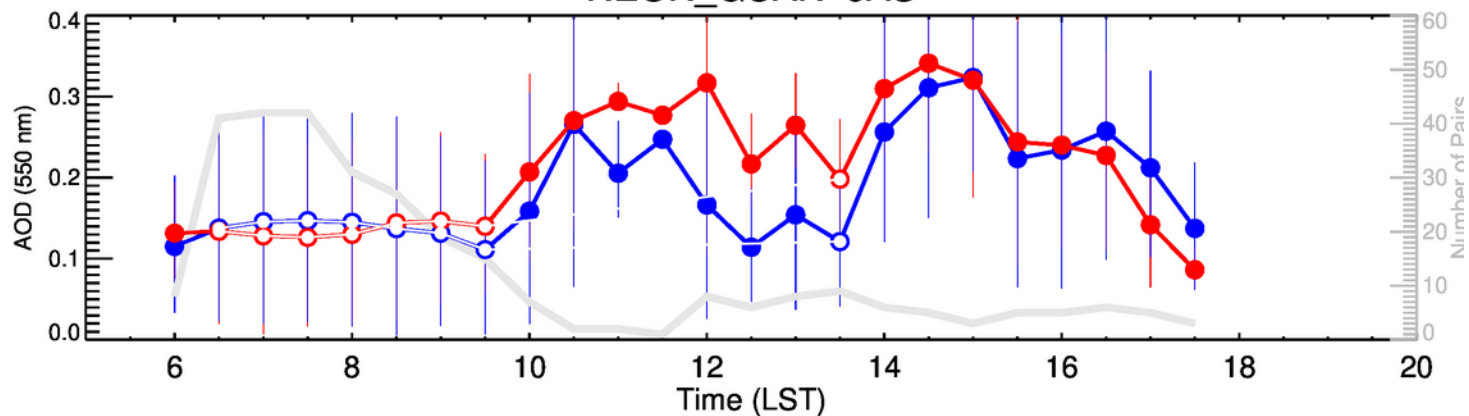
NEON_GUAN-OND
