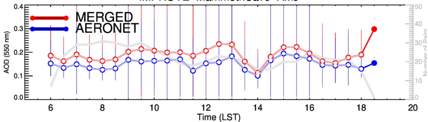
IMPROVE-MammothCave-JAS
