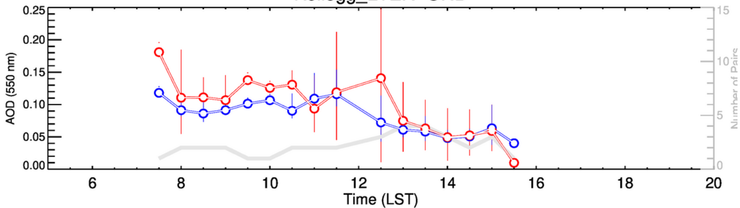
Kellogg_LTER-JFM
