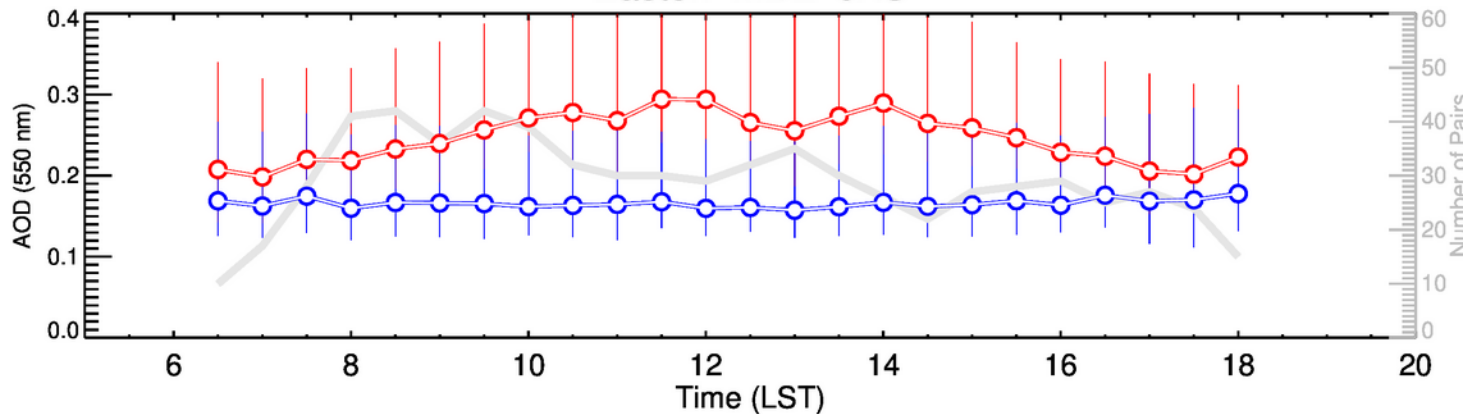
Easton-MDE-OND
