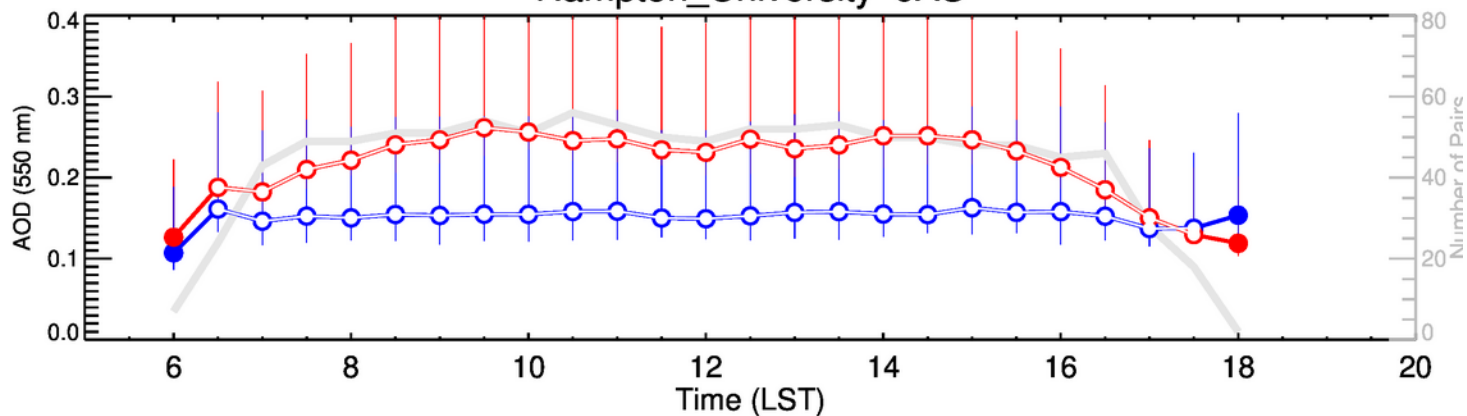
Hampton_University-OND
