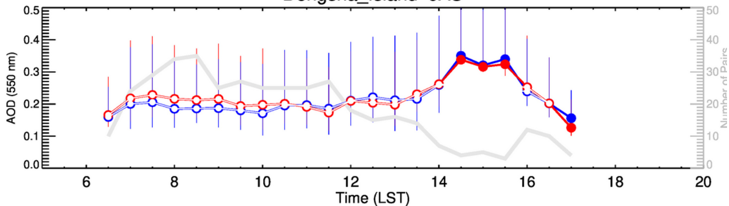
Dongsha_Island-OND
