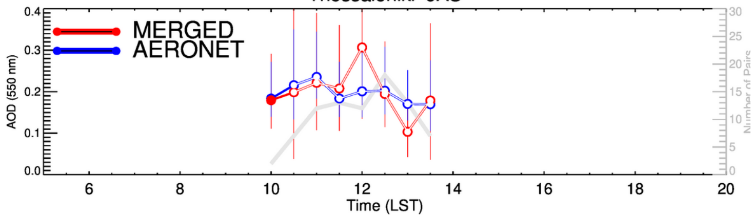
Thessaloniki-OND
