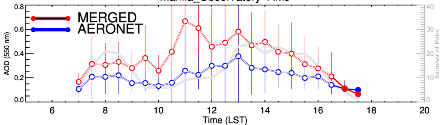
Manila_Observatory-JAS
