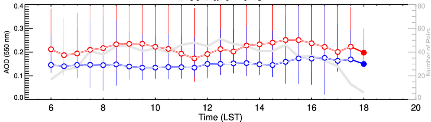
Brookhaven-OND
