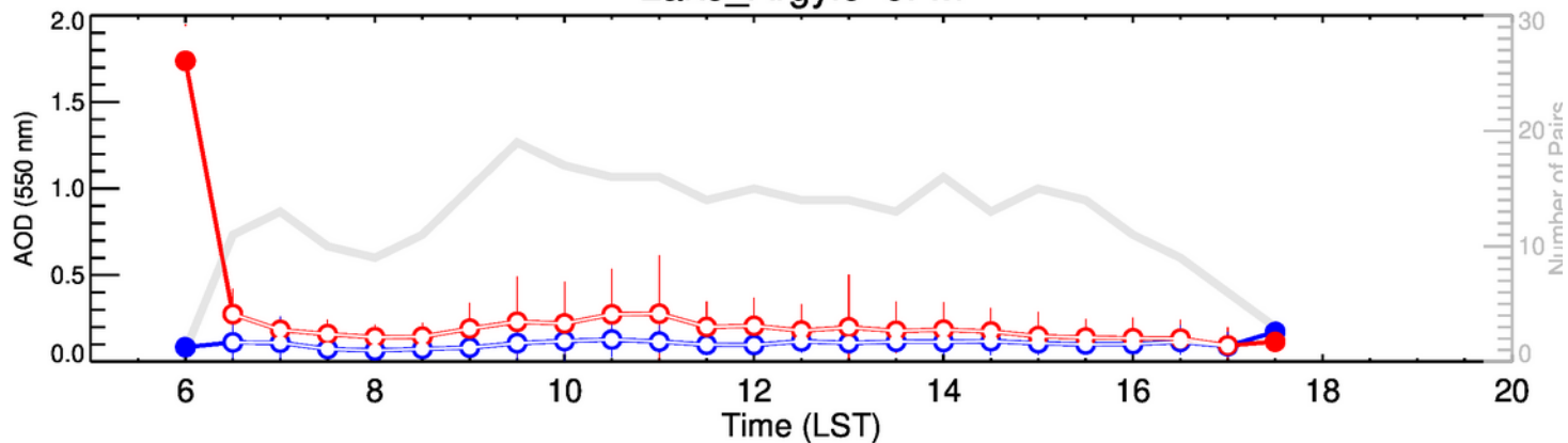
Lake_Argyle-JFM
