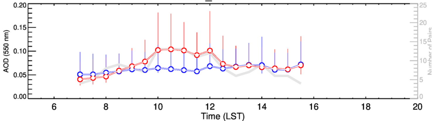
NEON_WREF-JFM
