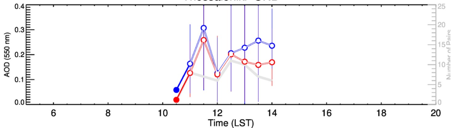
Thessaloniki-JFM
