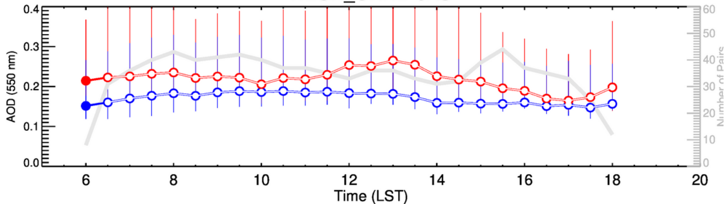
NEON_ORNL-OND
