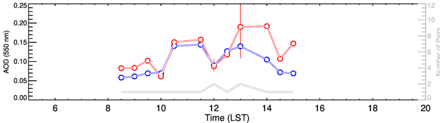
Easton-MDE-JFM
