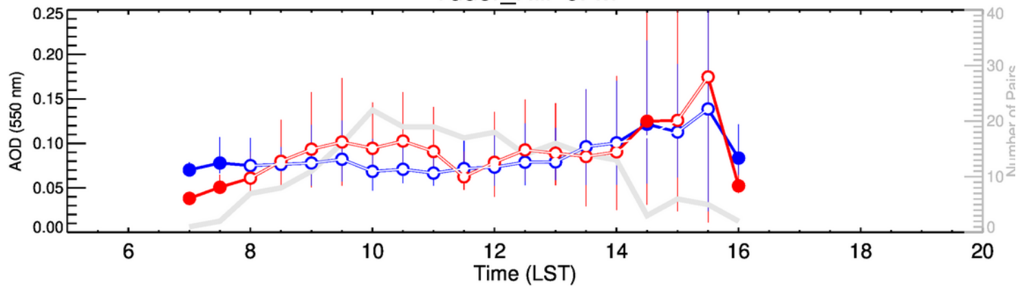
Tudor_Hill-JFM
