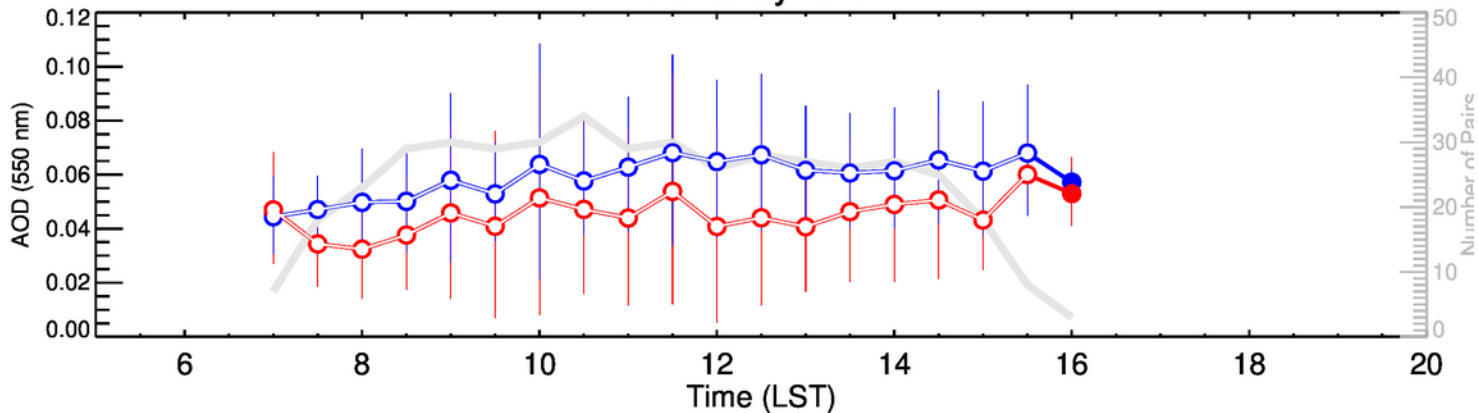
Monterey-JFM
