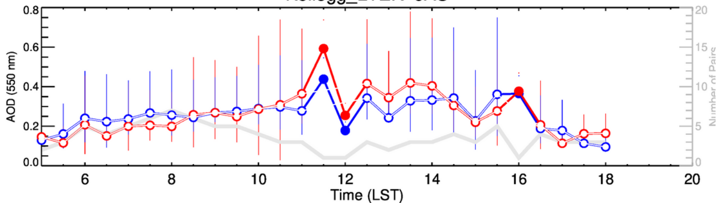
Kellogg_LTER-OND
