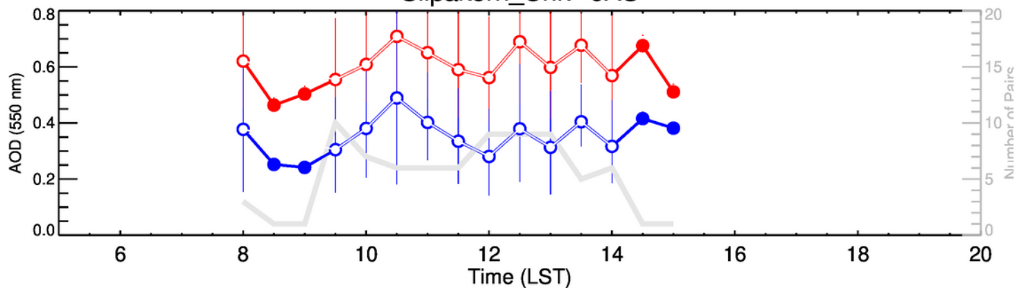
Silpakorn_Univ-OND
