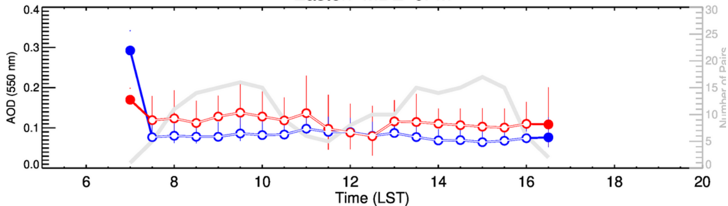
Easton-MDE-JFM
