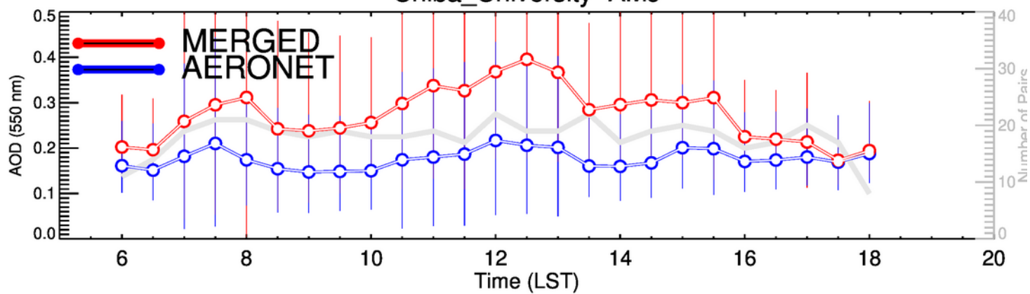
Chiba_University-JAS
