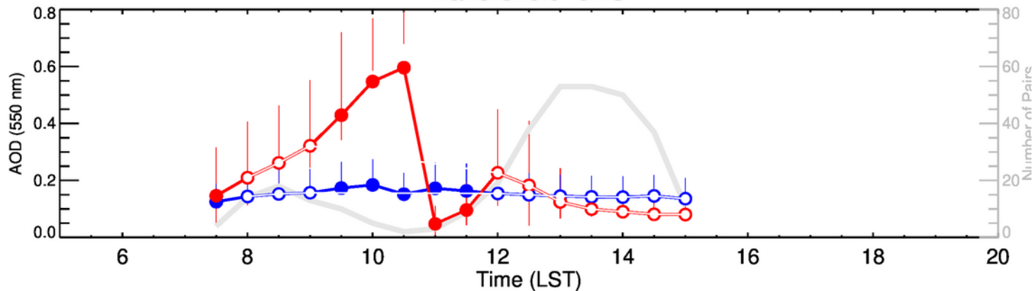
Bakersfield-OND
