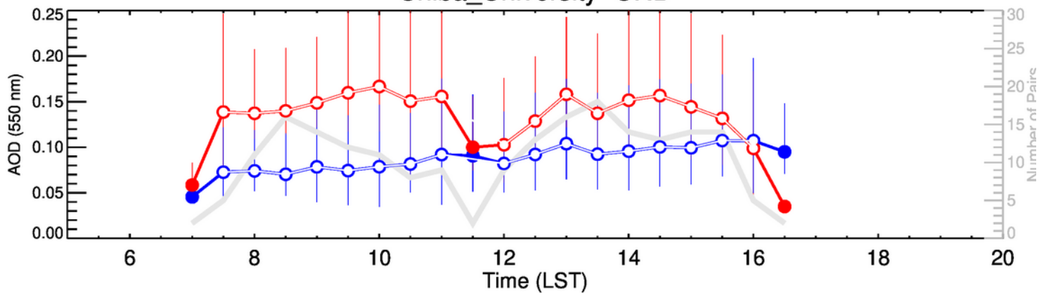
Chiba_University-JFM
