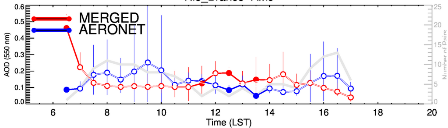
Rio_Branco-JAS
