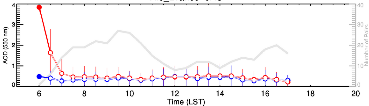
Rio_Branco-OND
