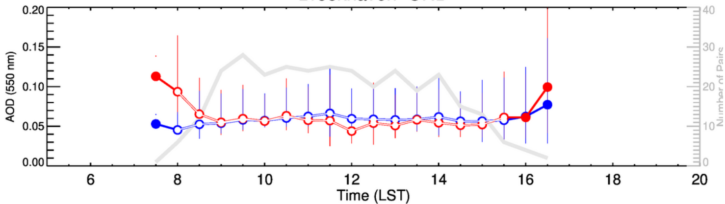
Brookhaven-JFM
