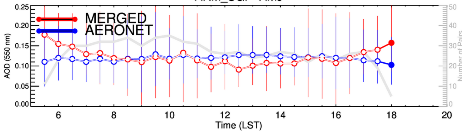
ARM_SGP-JAS
