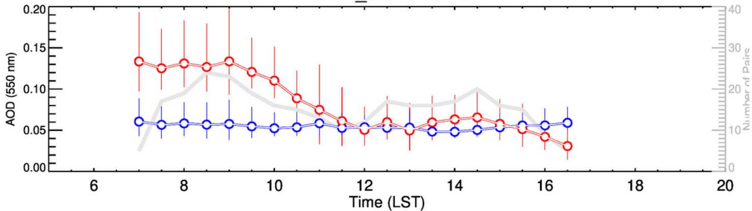
NEON_SERC-JFM
