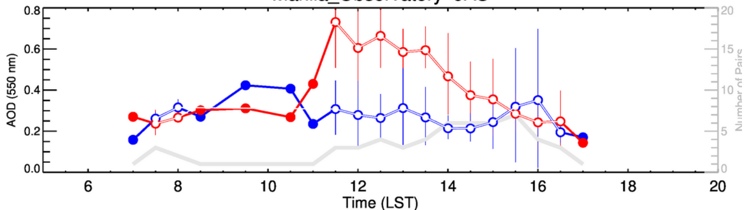
Manila_Observatory-OND
