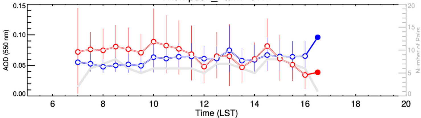
Thompson_Farm-JFM
