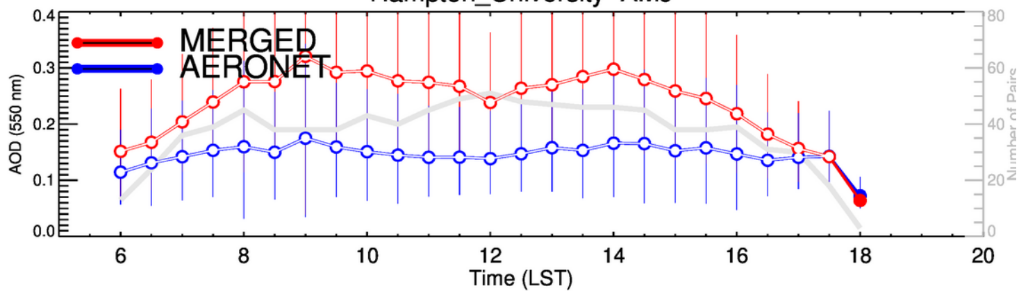
Hampton_University-JAS
