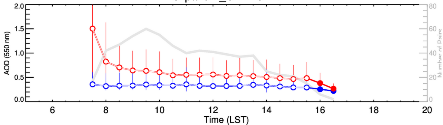
Silpakorn_Univ-JFM
