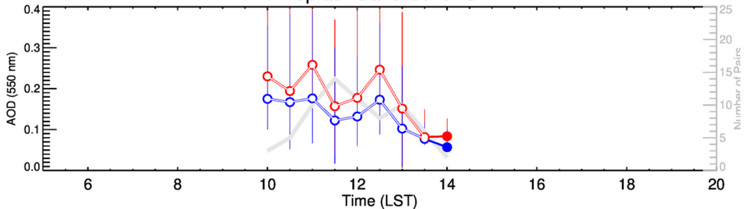
Poprad-Ganovce-OND
