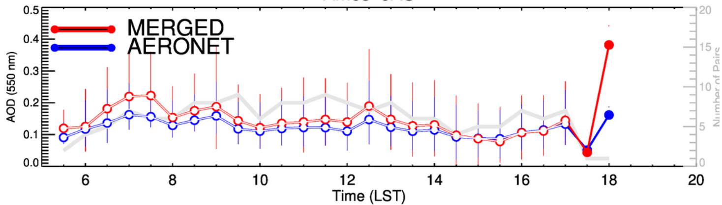
Ames-OND
