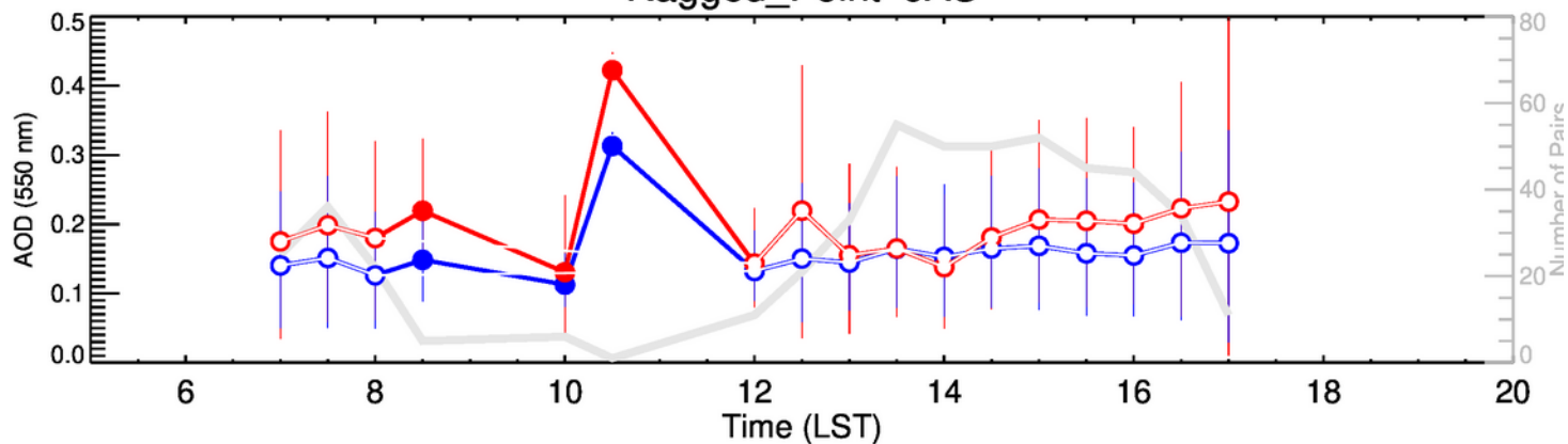
Ragged_Point-OND
