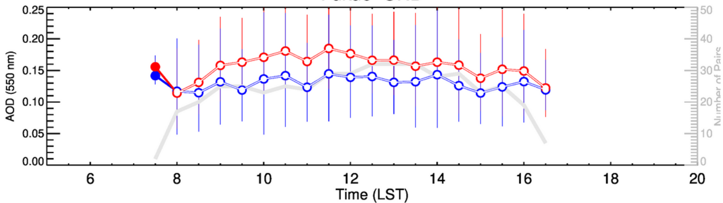
Fukue-JFM
