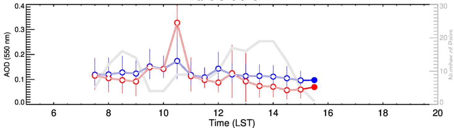
Bakersfield-JFM
