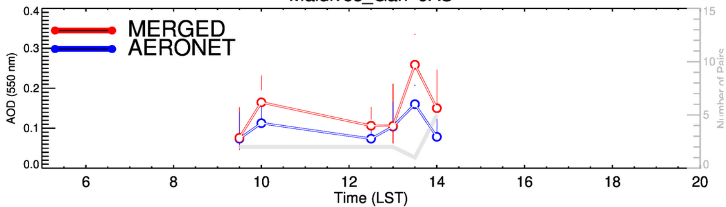
Maldives_Gan-OND
