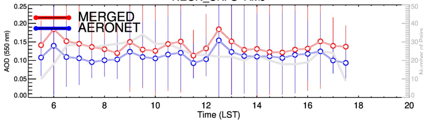
NEON_UKFS-JAS
