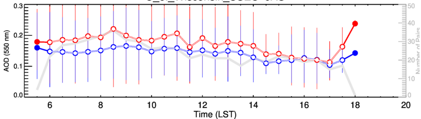
U_of_Wisconsin_SSEC-OND
