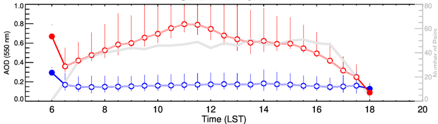
CEILAP-BA-JFM
