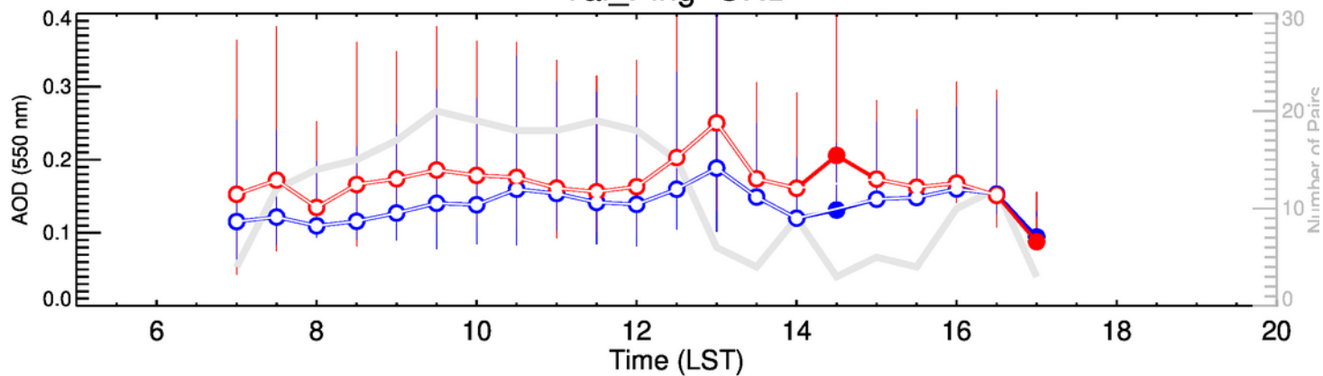
Tai_Ping-JFM
