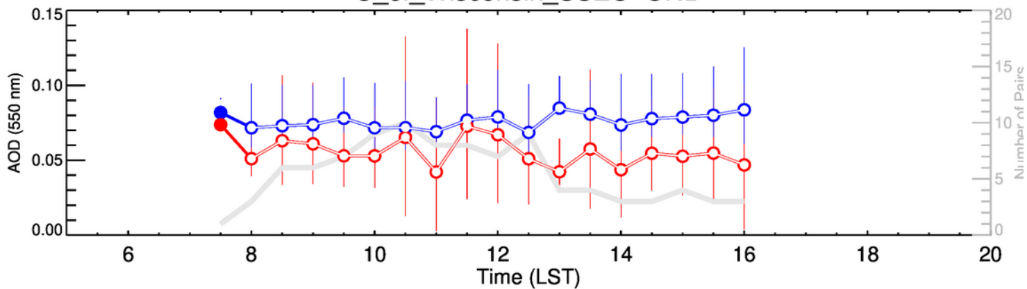
U_of_Wisconsin_SSEC-JFM
