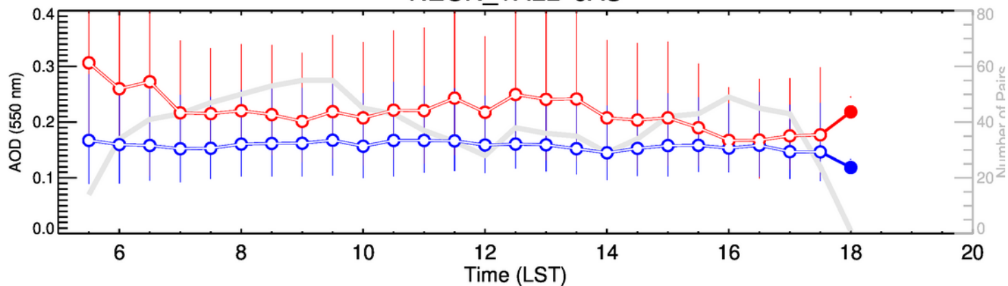
NEON_TALL-OND
