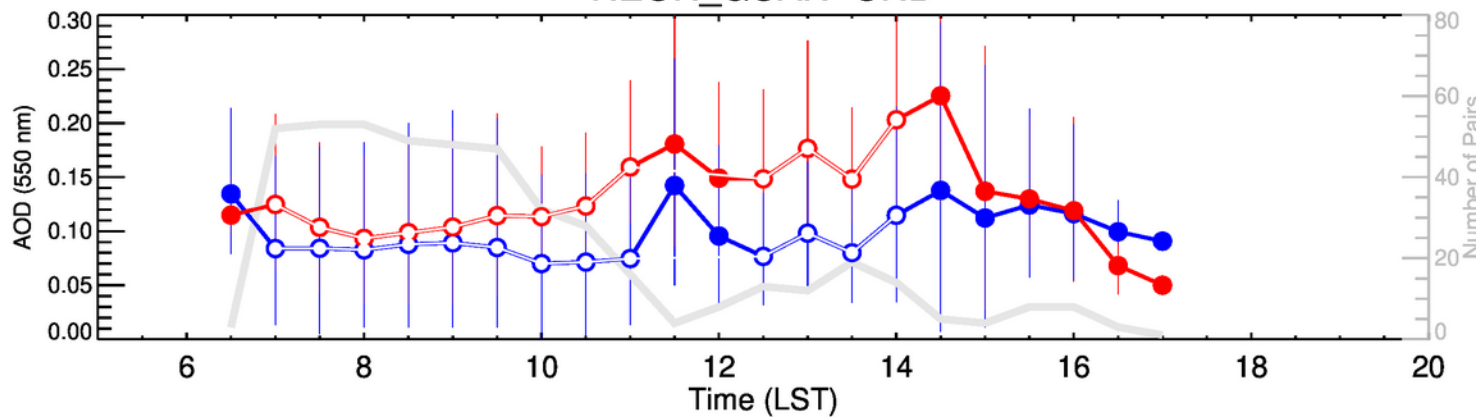
NEON_GUAN-JFM
