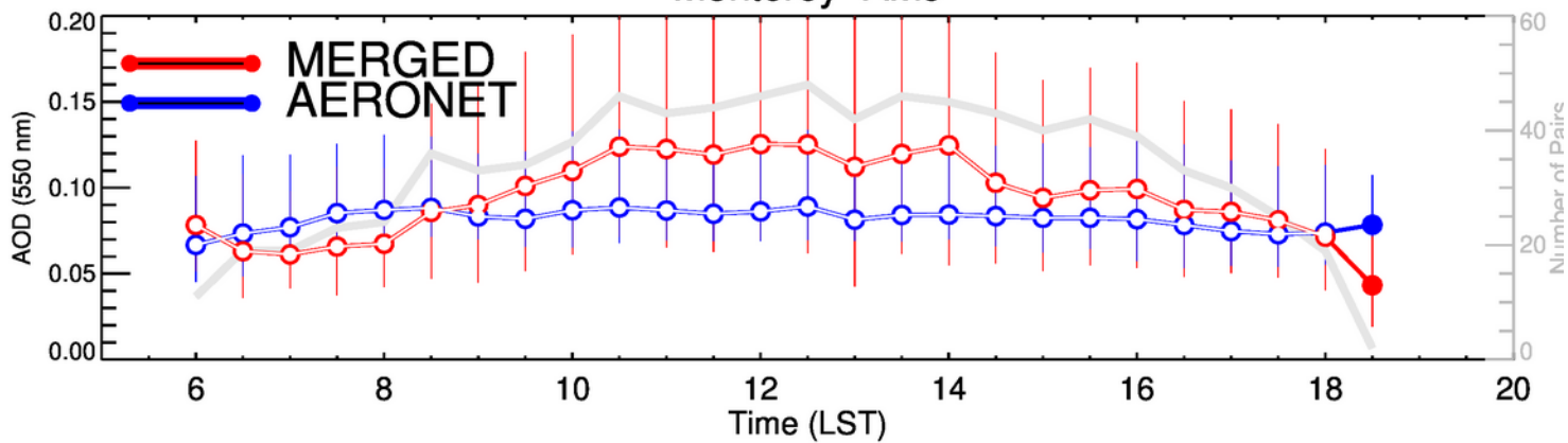
Monterey-JAS
