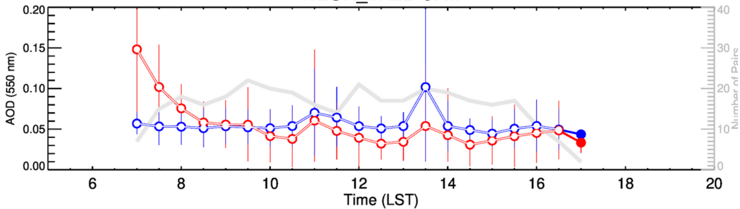
NEON_TALL-JFM
