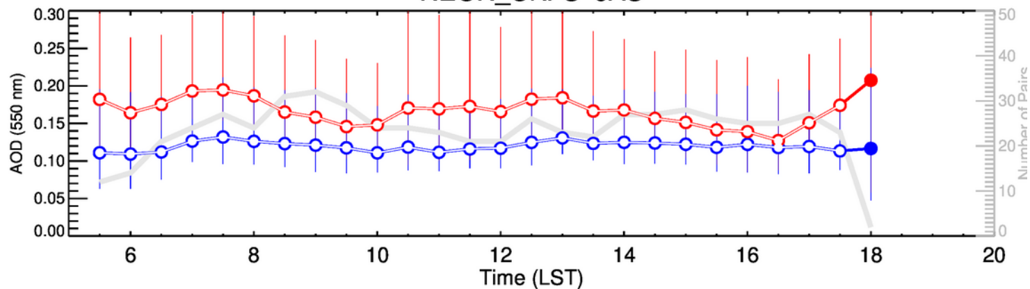
NEON_UKFS-OND
