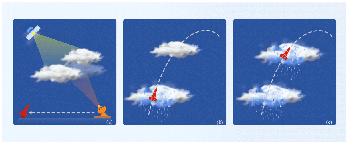
Figure 4. Schematic diagram of the working demo of a temporally controllable spatial seeding rocket.
