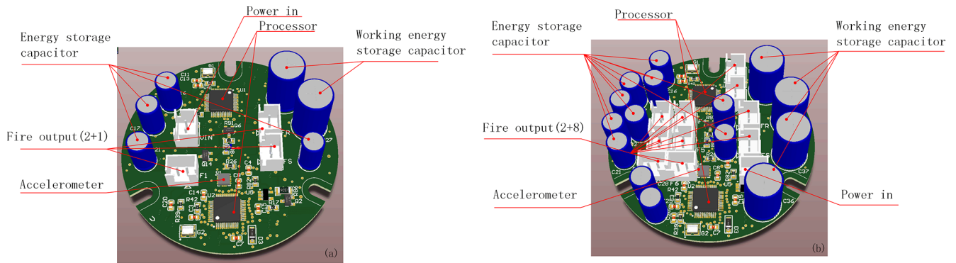
Figure 3. Three-dimensional model diagrams of the electronic fuses of (a) the ZBZ-HJ-7 spatial seeding rocket and (b) the temporally controllable spatial seeding rocket.
