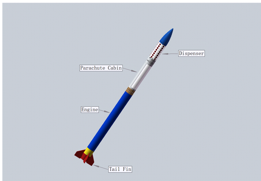
Figure 1. Schematic diagram of the ZBZ-HJ-7 spatial seeding rocket.
