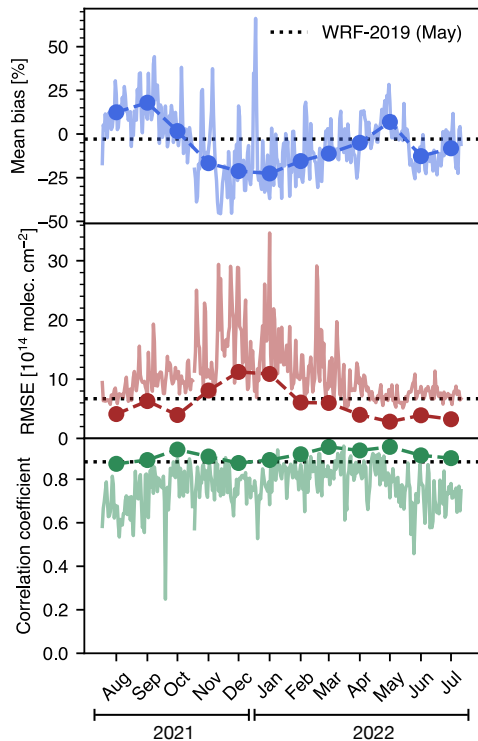
(a) NitroNet vs. TROPOMI
