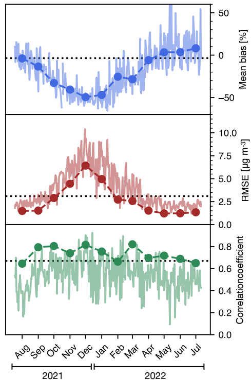
(b) NitroNet vs. AirBase
