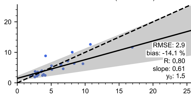
NitroNet vs. AirBase (Italy)
