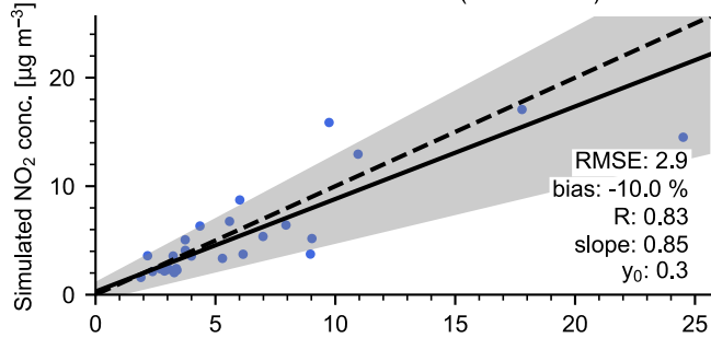
WRF-Chem vs. AirBase (Italy)
