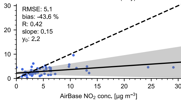
NitroNet vs. AirBase (Italy)
