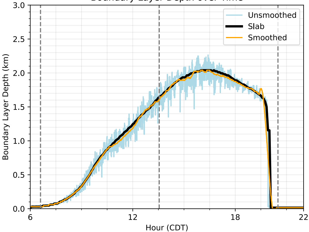
Boundary Layer Depth over Time
