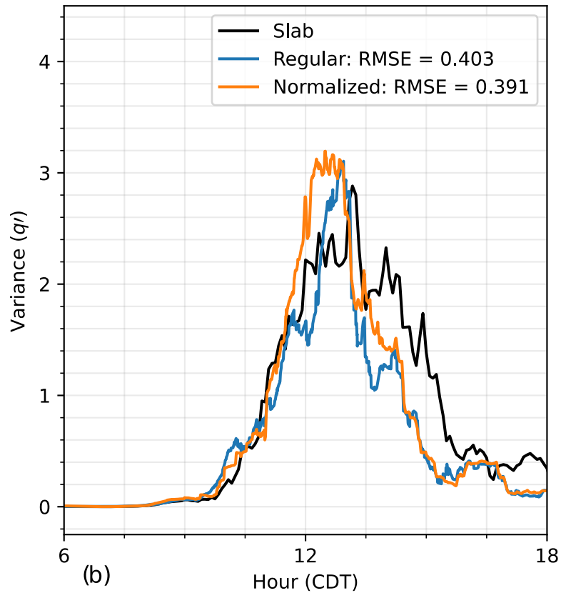
Top of the Boundary Layer
