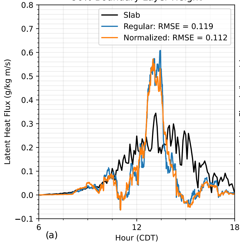
90% Boundary Layer Height
