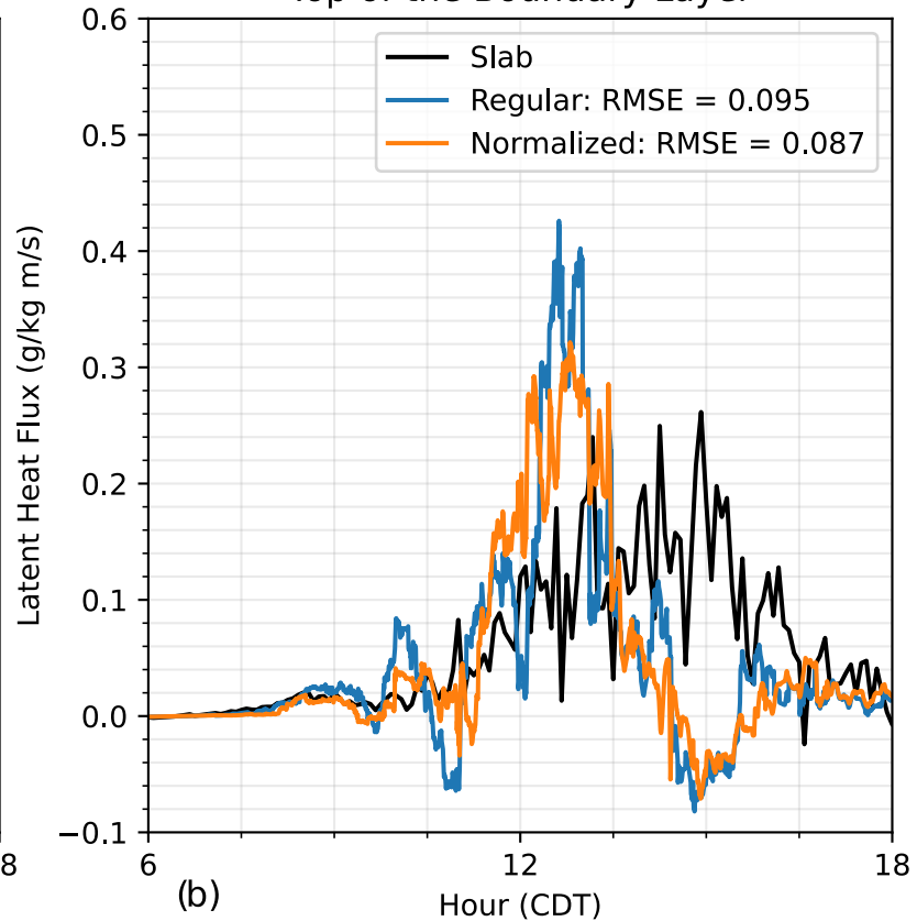
Top of the Boundary Layer
