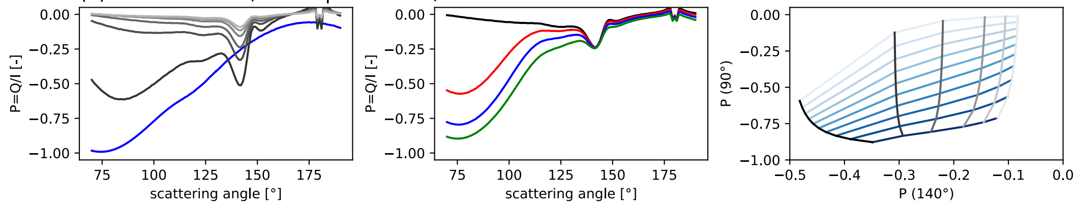
(a) ocean surface, wind speed = 5m/s
