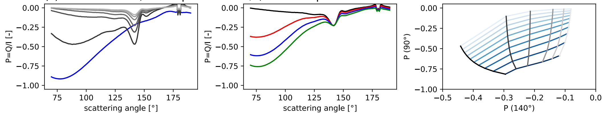
(c) ocean surface, wind speed = 10m/s, aerosol optical thickness = 0.1
