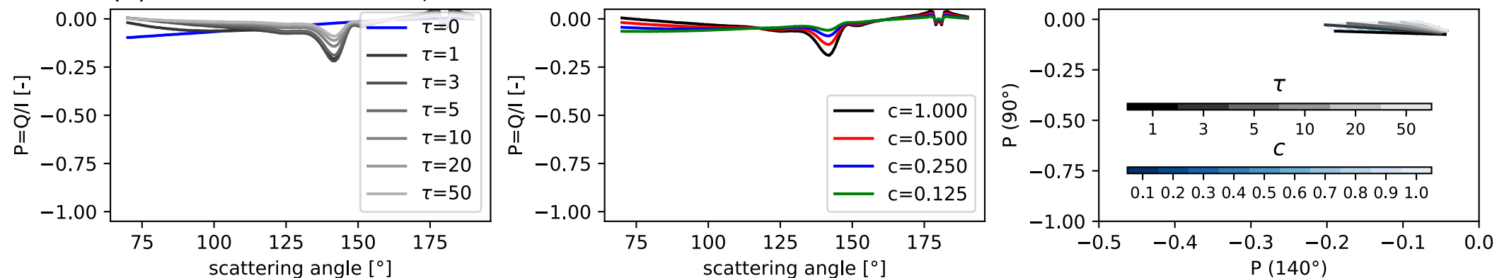
(e) Lambertian surface, albedo=0.2
