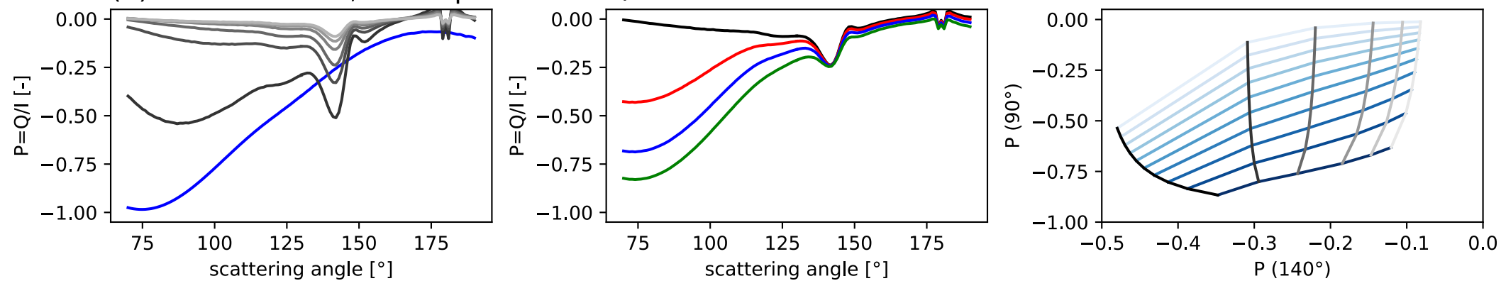
(b) ocean surface, wind speed = 10m/s
