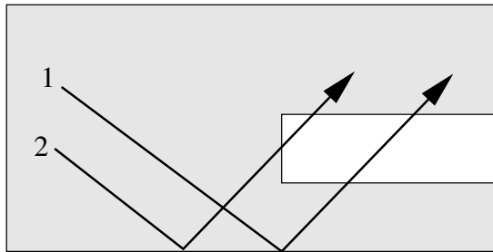
sun-glint
