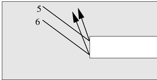
cloudbow
