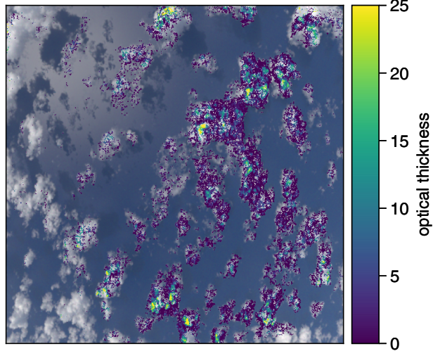
(a) optical thickness at stereo height
