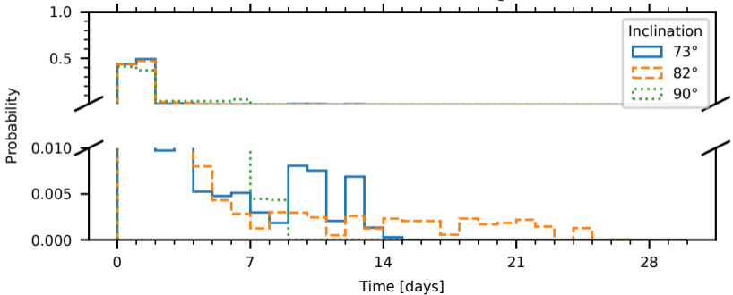
Distribution of bin return times for different orbital inclinations Bins: 5.0^\circ lat, 5.0^\circ long
