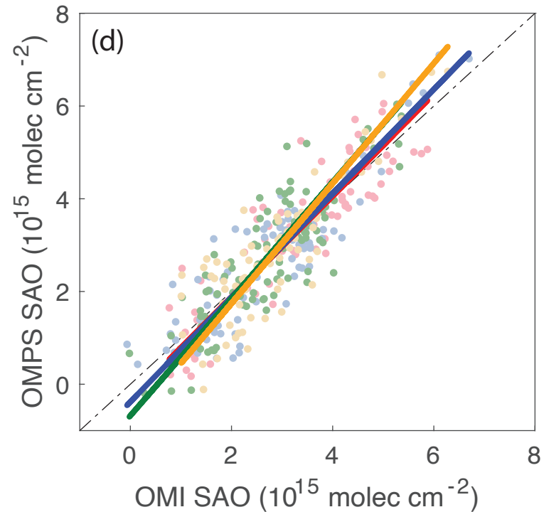
HCHO vertical column
