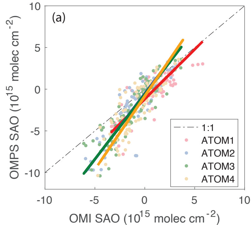
HCHO differential slant column
