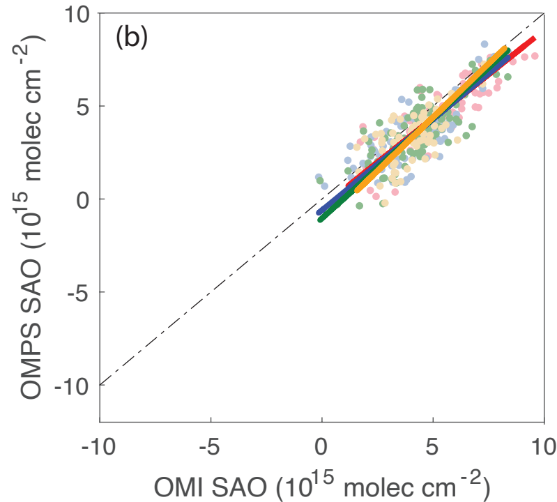
HCHO corrected slant column
