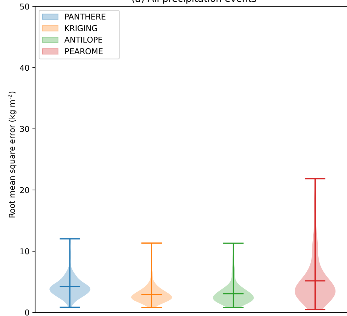
(a) All precipitation events
