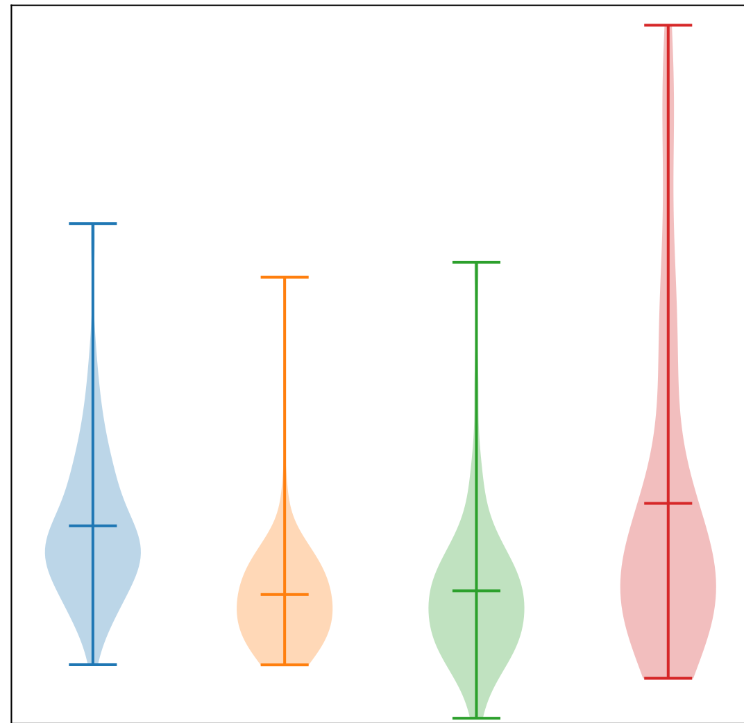
(b) Precipitation events above 10 \text{ kg m}^{-2} / 24 \text{ h}
