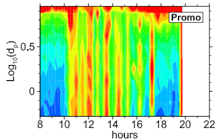
(c) Kurtosis
