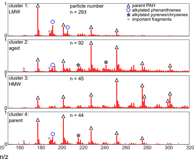
(b) Cluster analysis of LD-REMPI PAH mass spectra with Er:YAG laser used for LD
