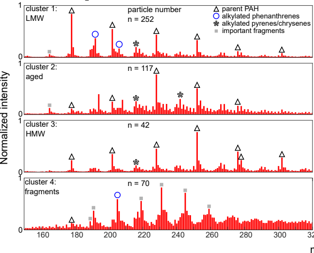
(a) Cluster analysis of LD-REMPI PAH mass spectra with CO 2 laser used for LD
