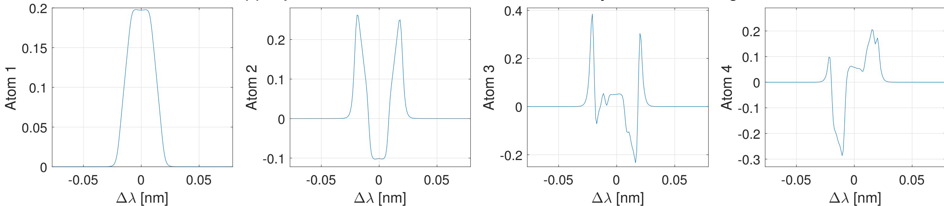
(b) Representation of the first atoms in the dictionary constructed using K-SVD
