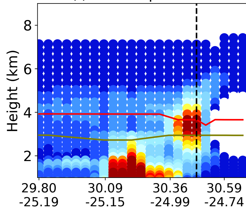
(f) Cloud liquid water
