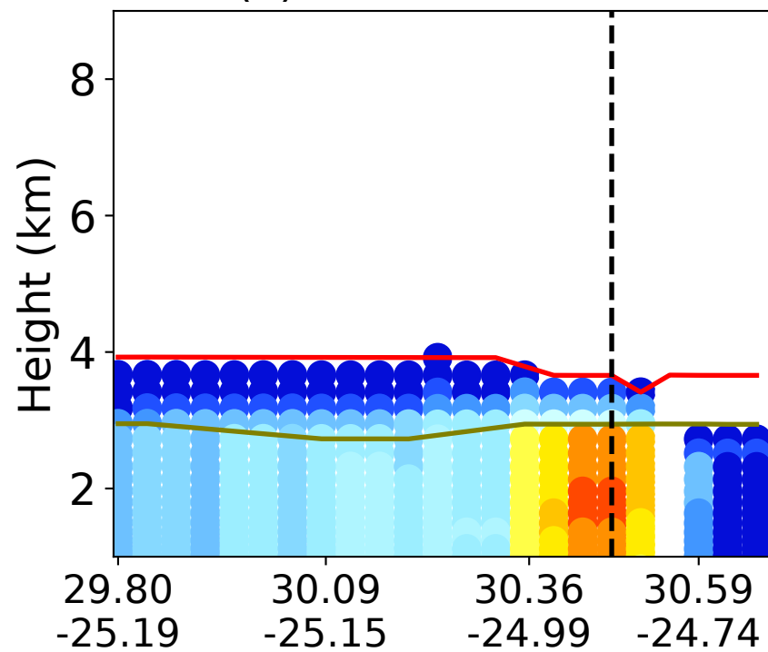
(e) Convective Rain
