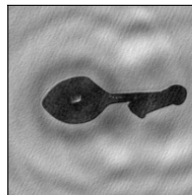
Lollipop_aggregate
