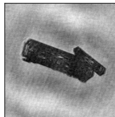
Column_aggregate
