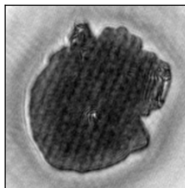
Droplet_aged
