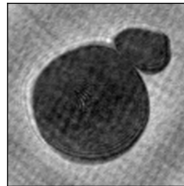
Droplet_aggregate
