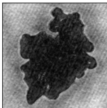
Irregular
