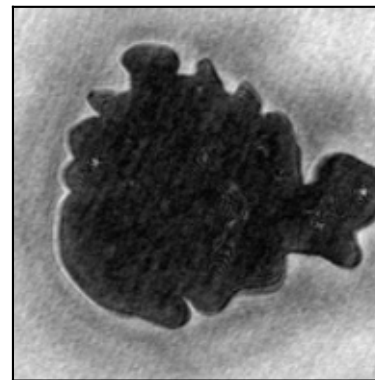
Droplet_aged_aggregate
