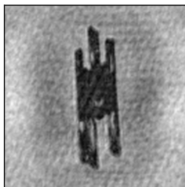
Column_plate
