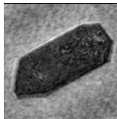
Plate
