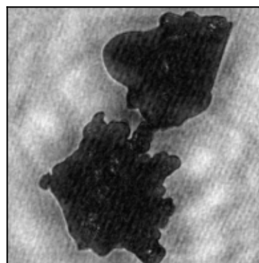
Irregular_aggregate
