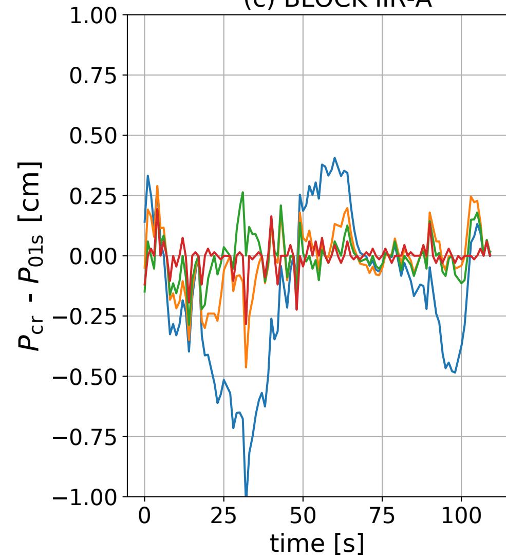
(c) BLOCK IIR-A
