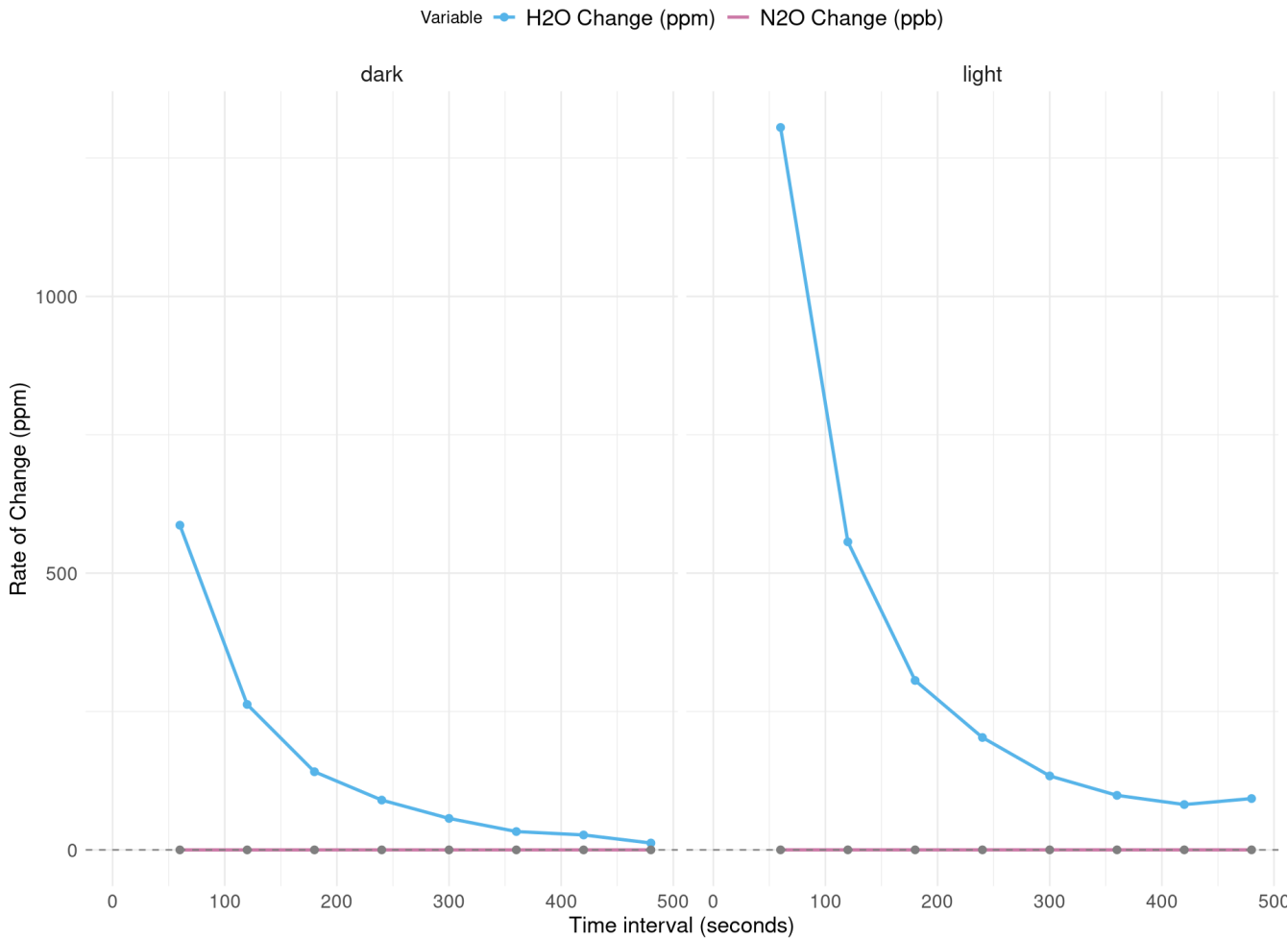
Figure S5. Rate of change on H2O and N2O concentration change during chamber closure times. The rate of change is calculated by subtracting the previous time stamp from the current, i.e. , rate of change = H2O concentration at (t+1) - H2O concentration at t. The left facet shows results for "dark measurements" only; the right for "light measurements". The line shows the 0 intercept.
