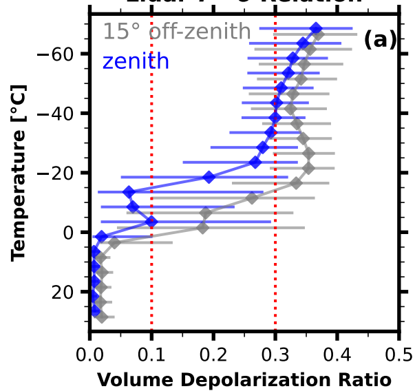
Lidar T - \delta Relation
