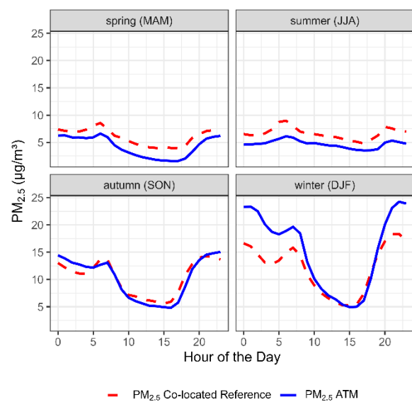
Figure S2. Hourly averaged uncorrected ( PM_{2.5} ATM) PurpleAir data measured at the 4 co-location sites compared to the hourly averaged co-located reference data for each season.
