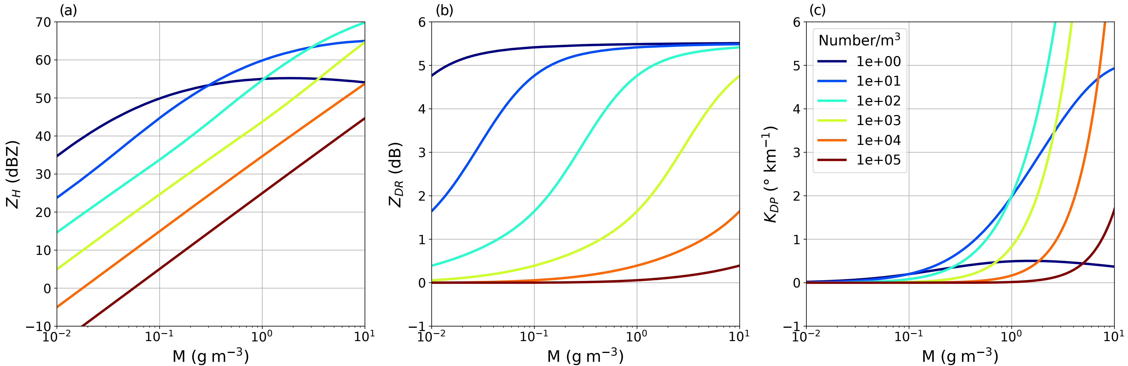
Z_H , Z_{DR} , K_{DP} as a function of M (in \text{g m}^{-3} ) C band, 2-moment PSD for rain, T=0^\circ\text{C}
