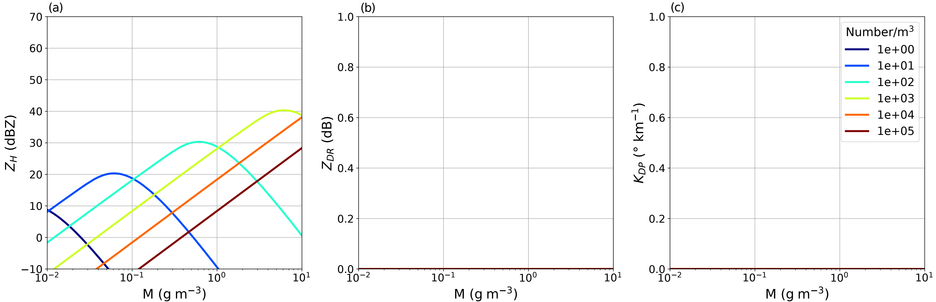
Z_H , Z_{DR} , K_{DP} as a function of M (in \text{g m}^{-3} ) C band, 2-moment PSD for ice, T=0^\circ\text{C}
