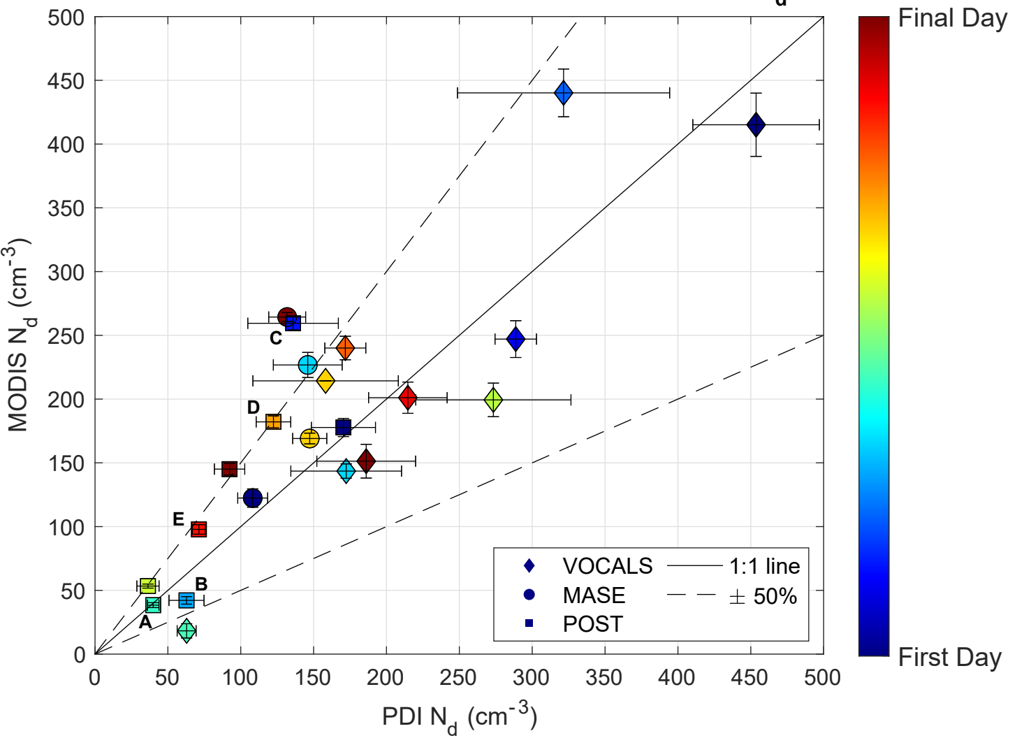
Comparison of MODIS vs. PDI number concentration ( N_d )
