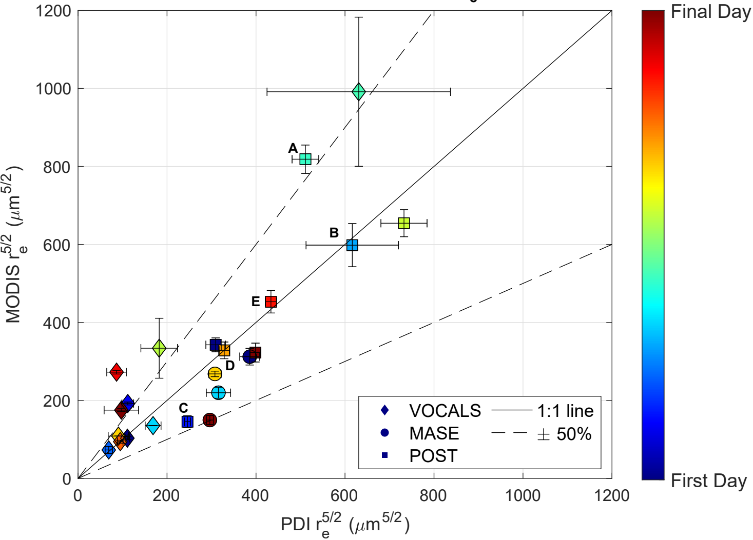
Comparison of MODIS vs. PDI r_e^{5/2}
