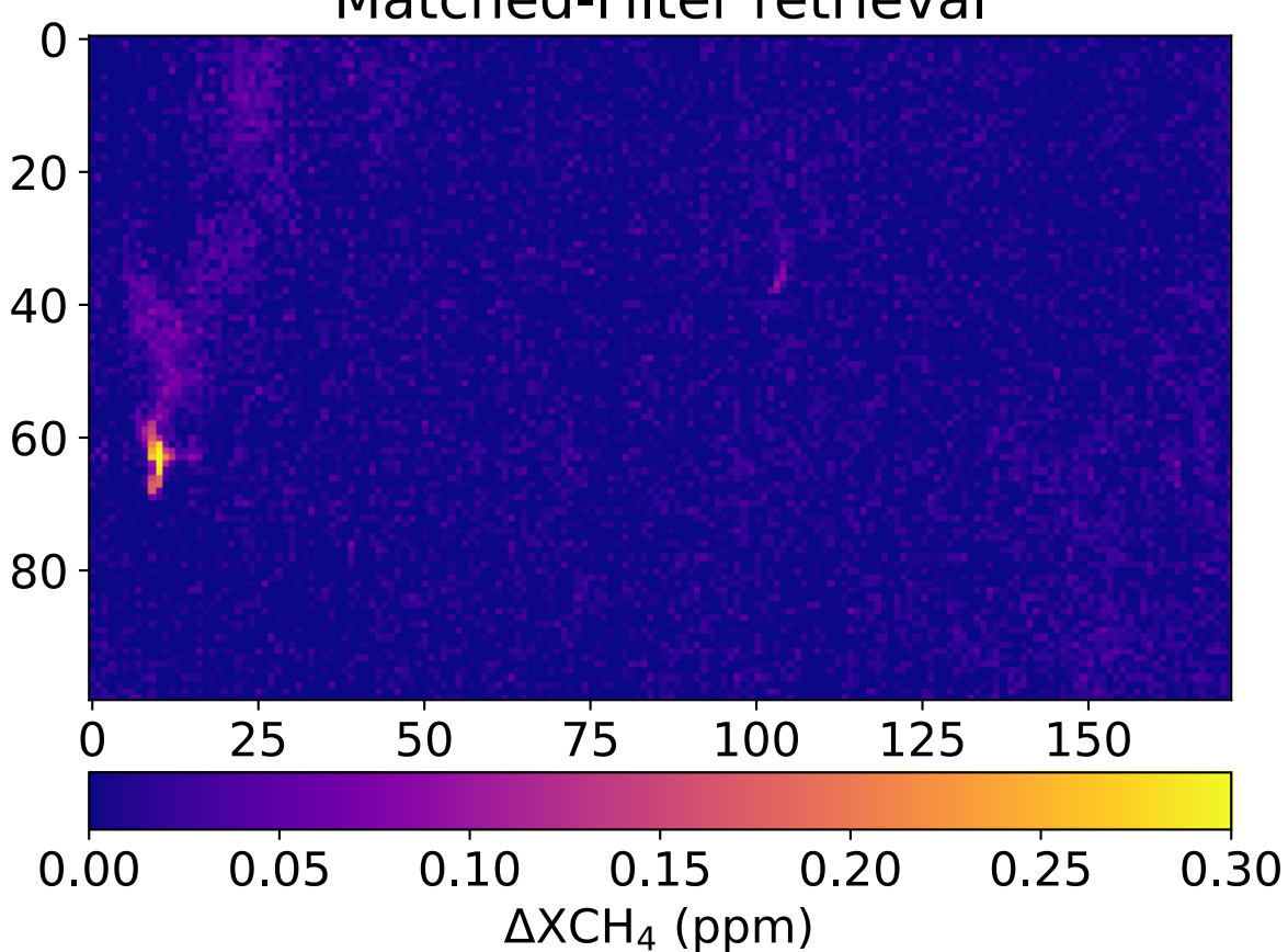
Matched-Filter retrieval
