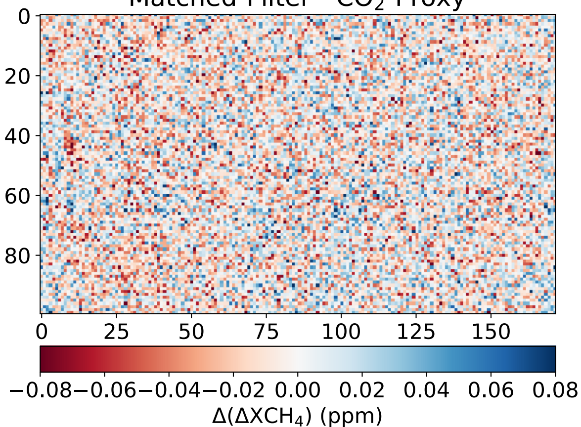
Matched-Filter - CO 2 -Proxy
