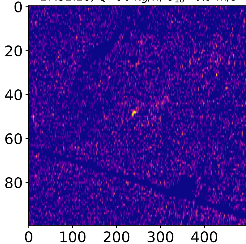
17:32:28, Q=96 kg/h, U_{10}=0.9 m/s
