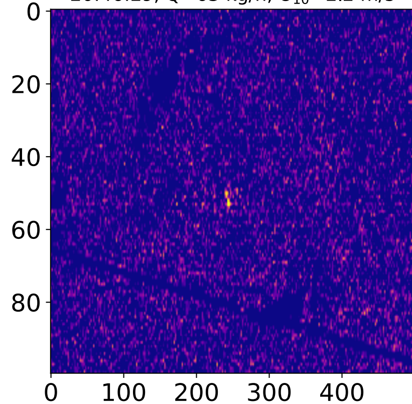
20:46:29, Q=63 kg/h, U_{10}=2.2 m/s
