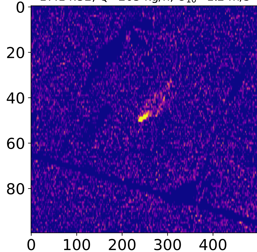
17:14:52, Q=205 kg/h, U_{10}=1.2 m/s
