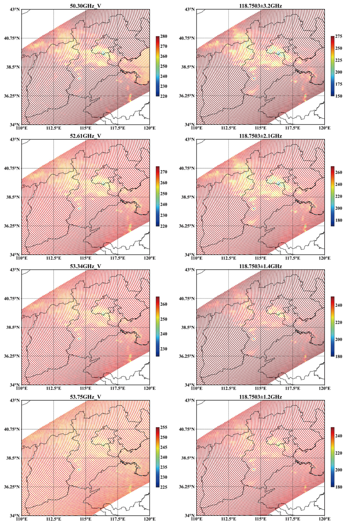
Figure B2. Similar to Fig. A2, but for the "07.2023" BTH extreme rainfall event (23:18 UTC, 30 July 2023).
