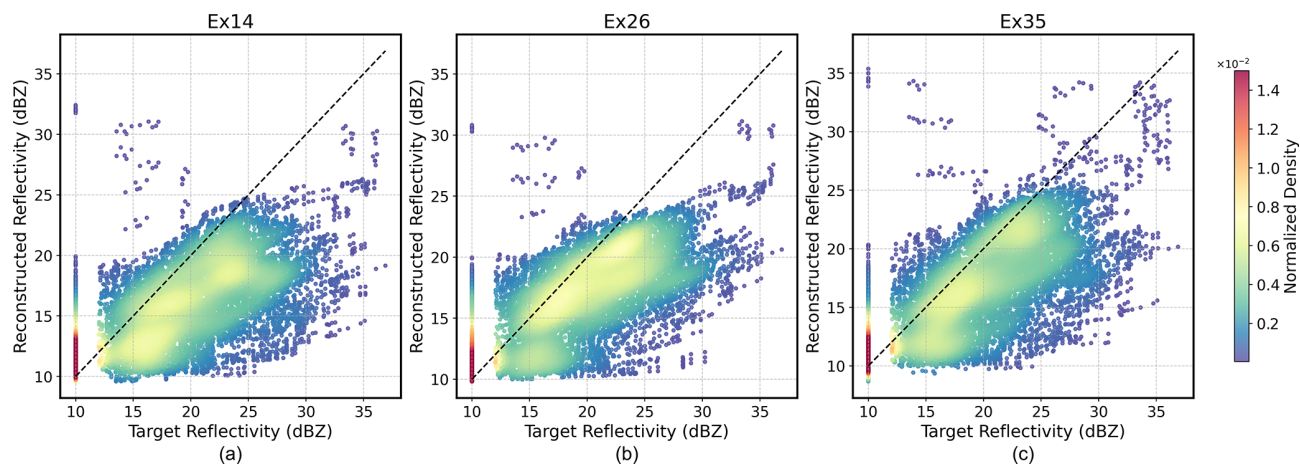
Figure 6. Similar to Fig. 4, but for the “07.2023” BTH extreme rainfall event (23:18 UTC, 30 July 2023).
