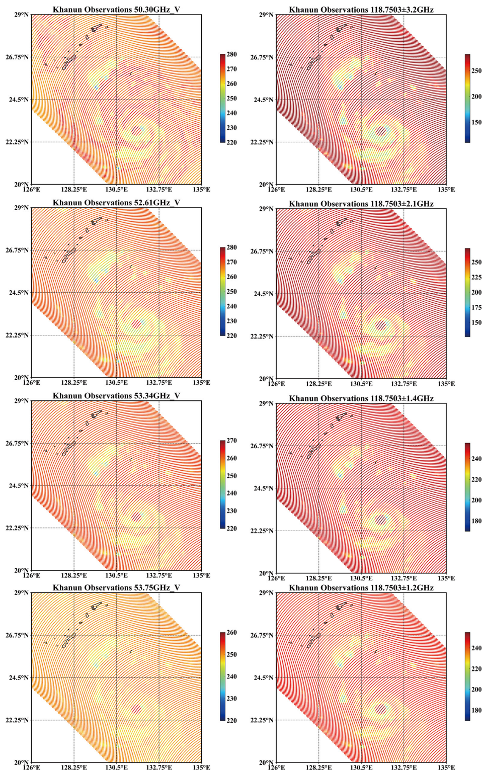
Figure B1. Spatial distributions of brightness temperatures observed by MWRI-RM for the oxygen absorption band channels during Typhoon Khanun (05:30 UTC, 31 July 2023).
