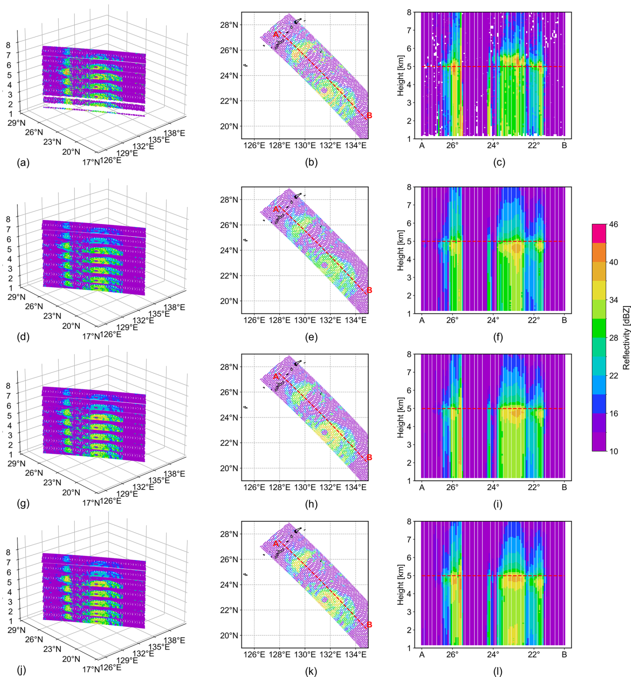
Figure 3. Comparative analysis of three-dimensional reflectivity structures of Typhoon Khanun (05:30 UTC 31 July 2023) across three experiments. The panels compare observed values (a–c) with reconstructed data from the Ex14 (e–f), Ex26 (g–i), and Ex35 (j–l) models. Each set includes 3D reflectivity structure (left), horizontal distribution at 5 km (middle), and vertical cross-section along points A and B (right).
