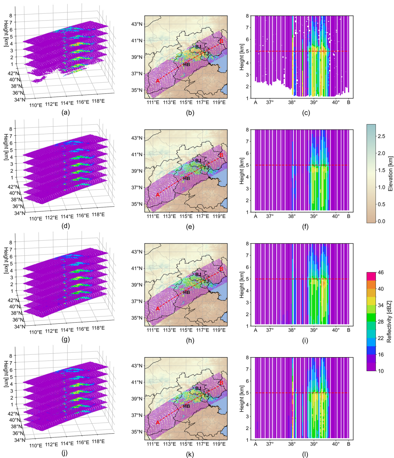
Figure 5. Similar to Fig. 3, but for the “07.2023” BTH extreme rainfall event (23:18 UTC, 30 July 2023). Panel (b) highlights the locations of Beijing (BJ), Tianjin (TJ), and Hebei (HB) provinces, labeled in black font.
