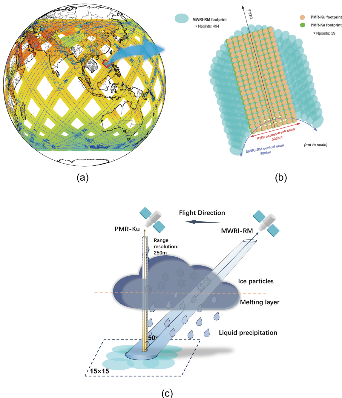
Figure 1. (a) The brightness temperatures from the MWRI-RM’s 52.61 GHz vertical polarization channel and PMR’s reflectivity at approximately 4 km above ground, recorded on 31 July 2023. The blue dashed line indicates the PMR scanning swath. (b) The viewing geometry of the MWRI-RM and PMR, with footprint sizes and numbers that do not correspond to actual observations but represent a conceptual example. “Npoints” refers to the number of scanning points along each scan line. Adapted from Fig. 1 in Turk et al. (2021). (c) Schematic representation of viewing volumes of MWRI-RM and PMR in the atmosphere, illustrating the patch extraction technique employed to match the footprint of MWRI-RM.
