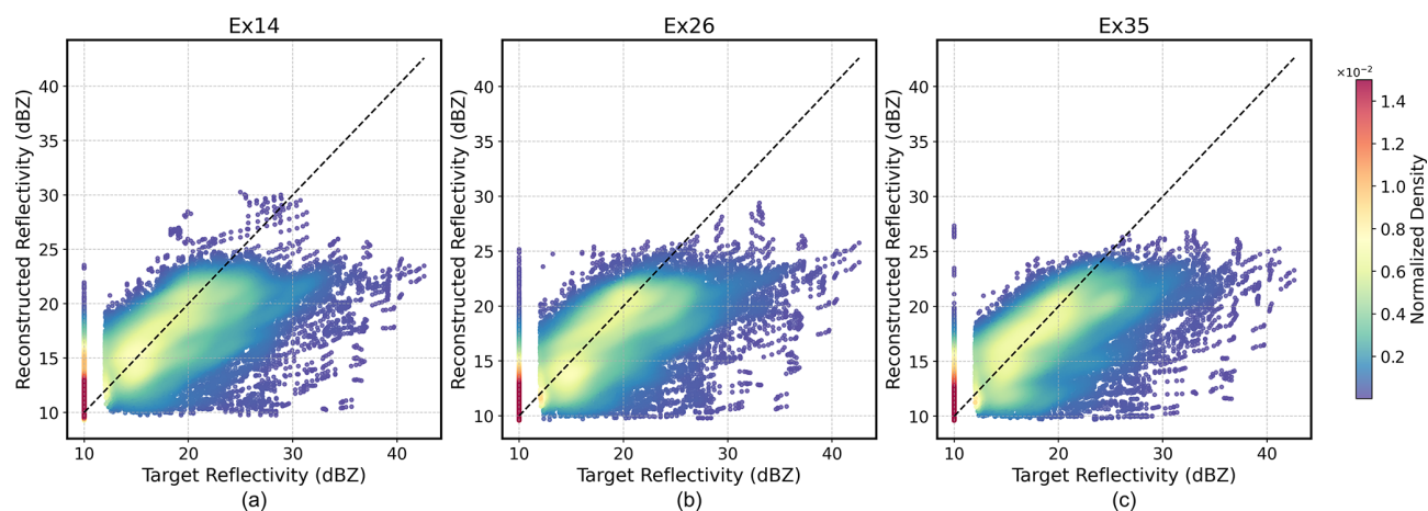
Figure 4. Scatter density comparison of observed and model-reconstructed reflectivity for Typhoon Khanun (05:30 UTC 31 July 2023) across three experiments. Data point density is represented by a color scale, with warmer colors (reds, yellows) indicating higher densities and cooler colors (blues, purples) indicating lower densities. The dashed diagonal line denotes perfect agreement (1 : 1 line) between observations and model estimates.
