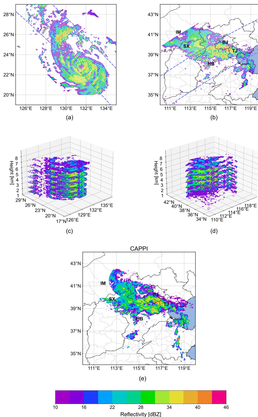
Figure 7. Ex35 model reconstructions of reflectivity from Typhoon Khanun (05:30 UTC 31 July 2023; left column) and the “07.2023” BTH extreme rainfall event (23:18 UTC 30 July 2023; right column) within the MWRI-RM swath. Panels (a), (b), and (e) depict the horizontal distribution at a 5 km altitude.
