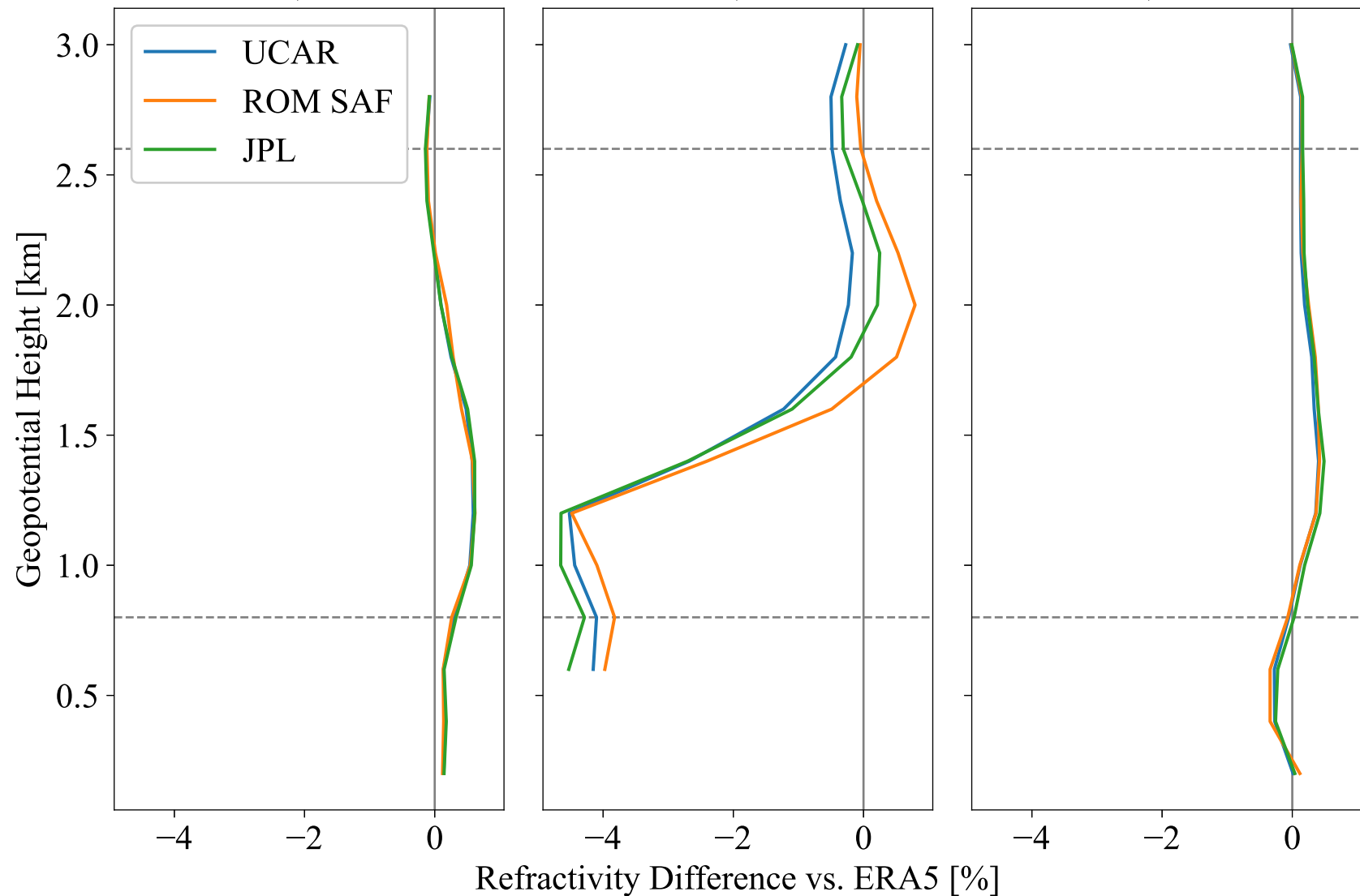
(b) Strong negative bias (stratocumulus)
