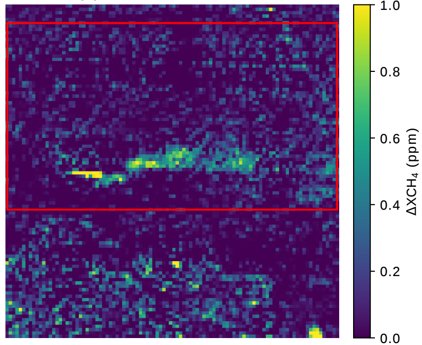
(b) PRISMA: 21/10/2021
