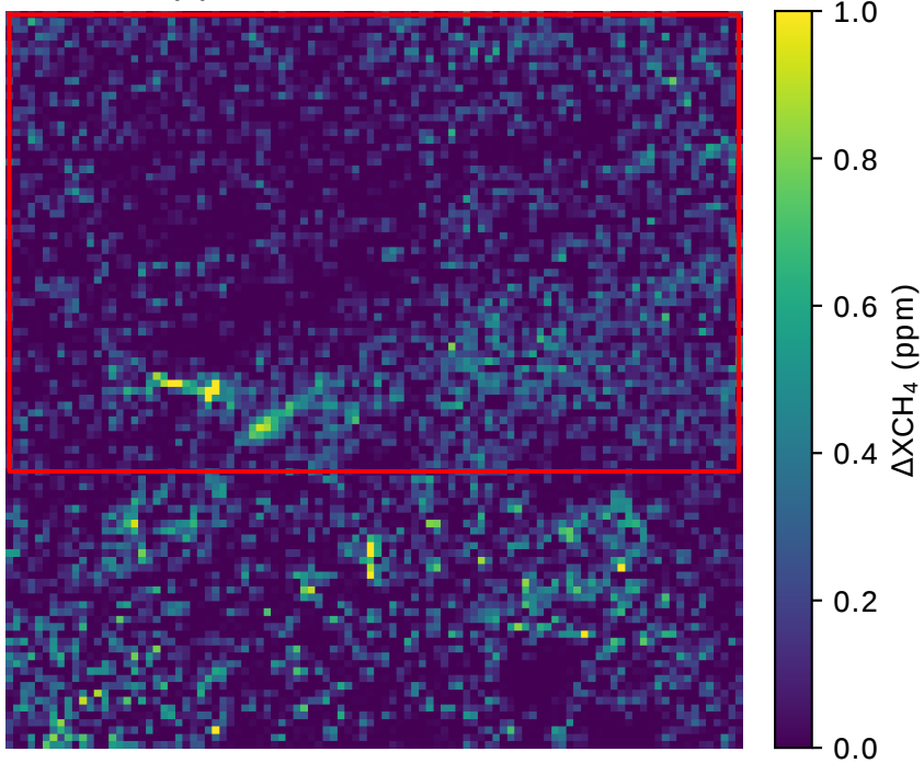
(c) PRISMA: 27/10/2021
