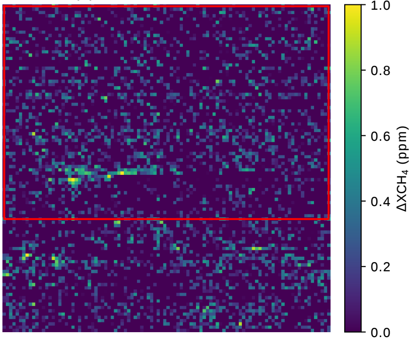
(a) PRISMA: 16/10/2021
