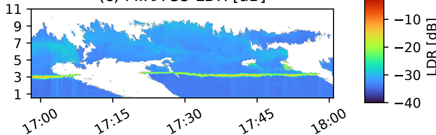
(c) MIRA-35 LDR [dB]
