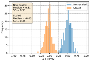
Pressure Level 0.53 hPa
