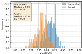
Pressure Level 1.1 hPa
