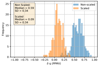
Pressure Level 0.25 hPa
