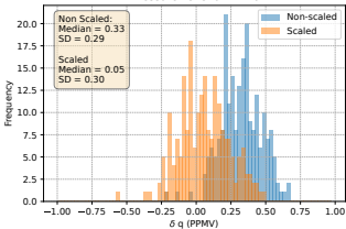
Pressure Level 0.12 hPa
