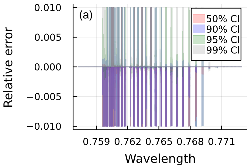
O2 Reconstruction
