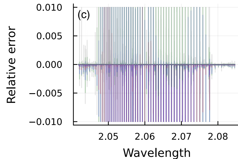
SCO2 Reconstruction
