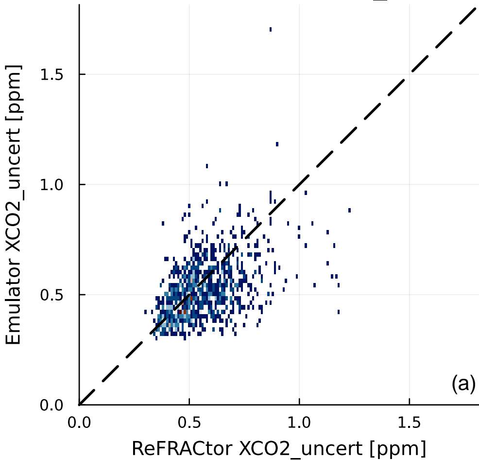
FP vs. Emulator XCO2_uncert
