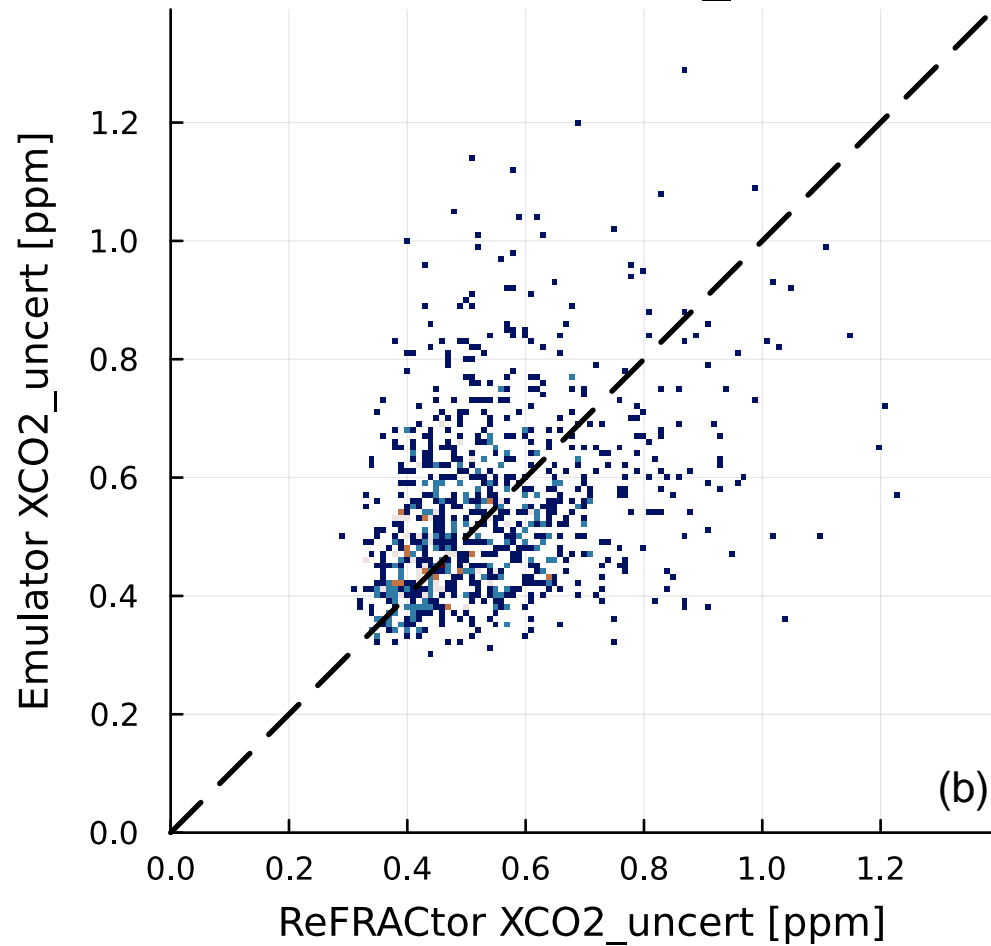
FP vs. Emulator XCO2_uncert (MD)
