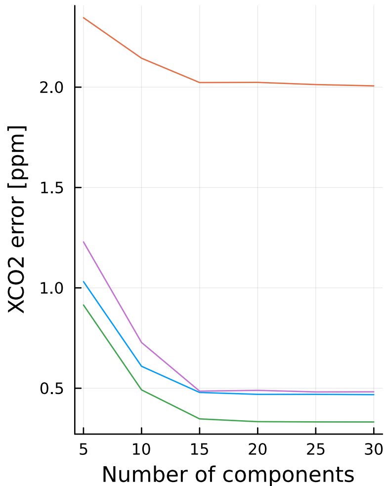
Retrieval MAE
