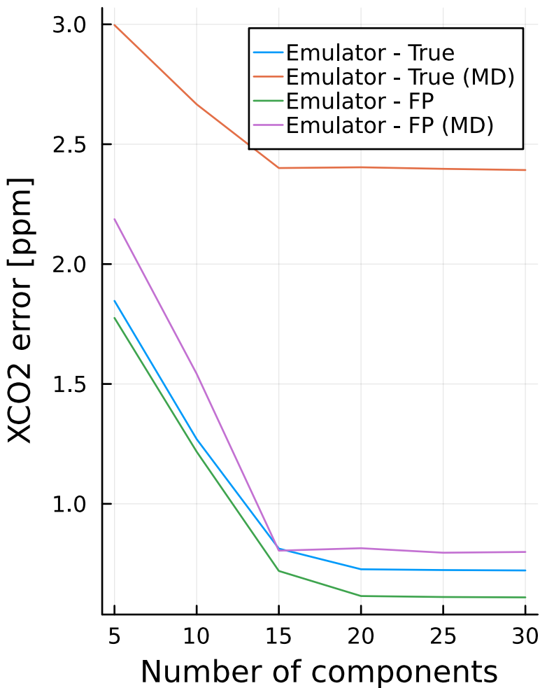
Retrieval RMSE
