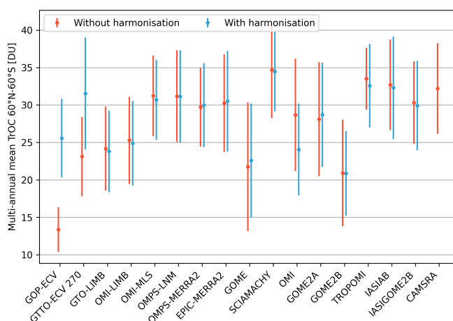
Figure 9. Near-global (60° N–60° S) multi-annual mean tropospheric ozone columns (TrOC) and dispersions before (red) and after (blue) harmonisation for all sixteen satellite data products and CAMSRA, over their full time series. The GTTO-ECV dataset covers 20° N–20° S and is not directly comparable to the near-global mean of the other datasets.
