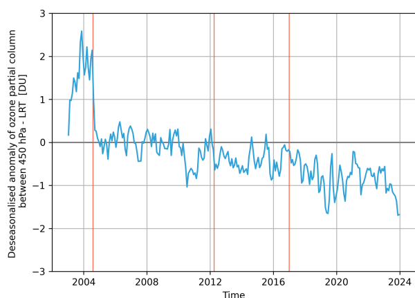
Figure 1. Difference (blue) between the derived climatology (2004–2016) and full reanalysis CAMS correction terms for going from the 450 hPa top level tropospheric column to the lapse-rate tropopause column. Vertical lines (red) indicate important changes in the CAMS assimilation system as detailed in Inness et al. (2019).
