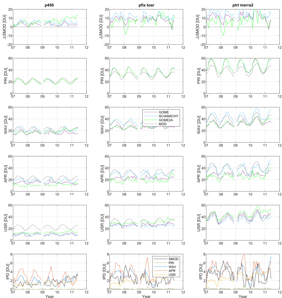
Figure 3. Evaluation of nadir ozone profile harmonisation for the overlapping period (January 2007–June 2011) of GOME (purple), SCIAMACHY (blue), and GOME-2A (green), restricted to their common spatiotemporal sampling. The first row shows the difference between the CAMSRA model data (black dashed lines) before and after averaging kernel smoothing. The second to fifth rows contain global mean tropospheric ozone time series for the prior profile columns (PRI), weighted-averaged retrieved columns (WAV), harmonised columns using a-priori profile replacement (APR), and columns in their unit-sensitivity representation (USR), respectively, all in DU. The last row depicts the IPD [DU] for each of the rows above. The PRI dispersion here roughly equals zero as all three products result from essentially the same RAL algorithm and prior input. The three columns correspond to the three selected tropospheric top level definitions.
