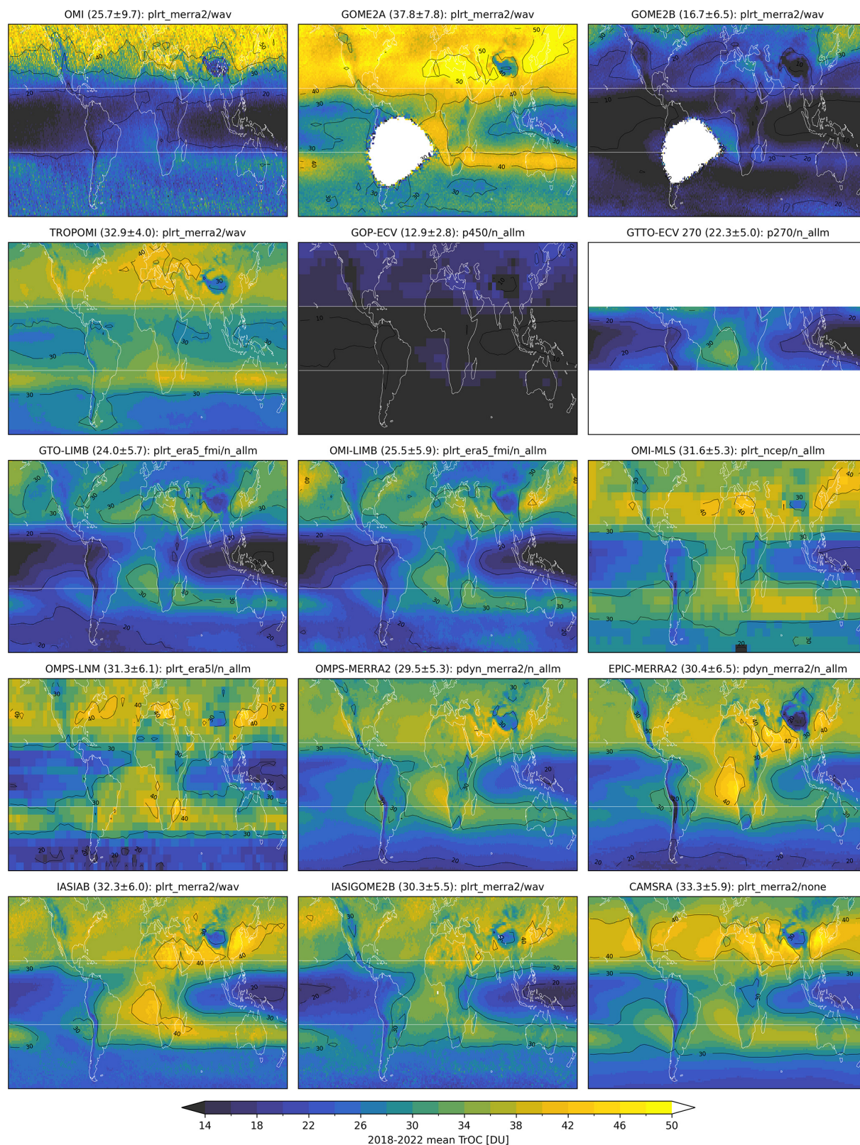
Figure 6. Multi-annual mean (2018–2022) tropospheric ozone column (TrOC) distribution of fourteen satellite data products and CAMSRA before harmonisation. Area-weighted mean and standard deviation of the near-global tropospheric column ( 60^{\circ} N– 60^{\circ} S) are given between brackets.
