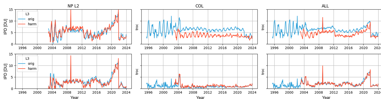
Figure 11. Inter-product dispersion (IPD) [DU] before (blue) and after (red) harmonisation, for the near-global time series of all sixteen satellite data products, both without (top) and with (bottom) their respective near-global means subtracted. The left and middle columns differentiate the results for all datasets (on the right) between the Level-2 profile products and the Level-3 column products, respectively.
