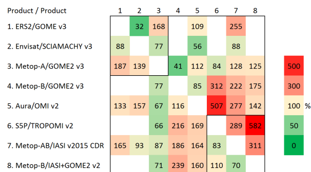
Figure 2. Spatiotemporally averaged relative difference between each product pair upon going from WAV to APR (below diagonal) and to USR (above diagonal), expressed in terms of the ratio, in %, between the products' mean difference before and after harmonisation, for all three top level definitions combined. For values below 100 % (in green), the harmonised product monthly means are closer to each other than the weighted averages, the opposite is true for the values above (in red). The diagonal and combinations without temporal overlap are empty. The top-left and bottom-right three-by-three boxes indicate the combinations that are used for Figs. 3 and 4, respectively.
