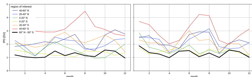
Figure 12. Zonal and near-global (60°N–60°S) seasonal cycles of the IPD [DU] for the full time series of all sixteen satellite data records, both before (left) and after (right) harmonisation. Note that the latter is limited to the CAMSRA temporal domain (2003–2023).
