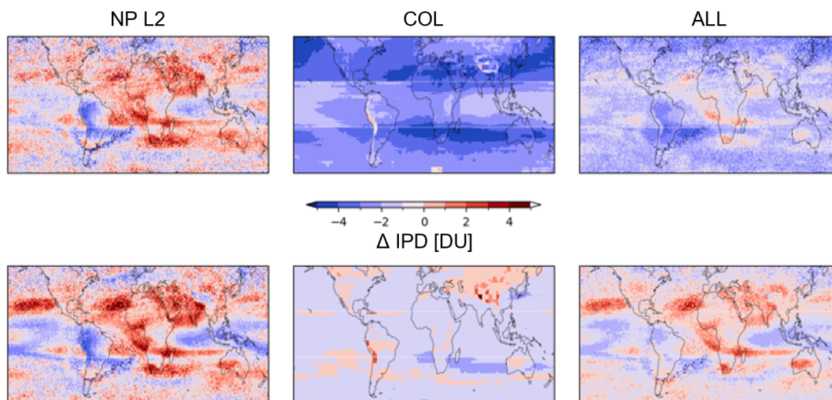
Figure 8. Change of the IPD (in DU) between satellite data sets upon harmonisation (after minus before), for the 2018–2022 mean of fourteen satellite data products. The top row shows the absolute tropospheric ozone column values, the bottom row their spatial anomaly (i.e. after subtraction of the 60° S–60° N mean). The left and middle columns differentiate the results for all fourteen datasets (on the right) between the Level-2 profile products and the Level-3 column products, respectively.
