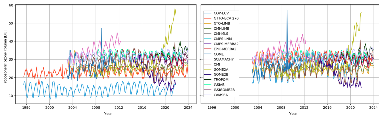
Figure 10. Near-global (60° N–60° S) tropospheric ozone column time series for all sixteen satellite data records and CAMSRA, both before (left) and after (right) harmonisation. Note that the latter is limited to the CAMSRA temporal domain (2003–2023).
