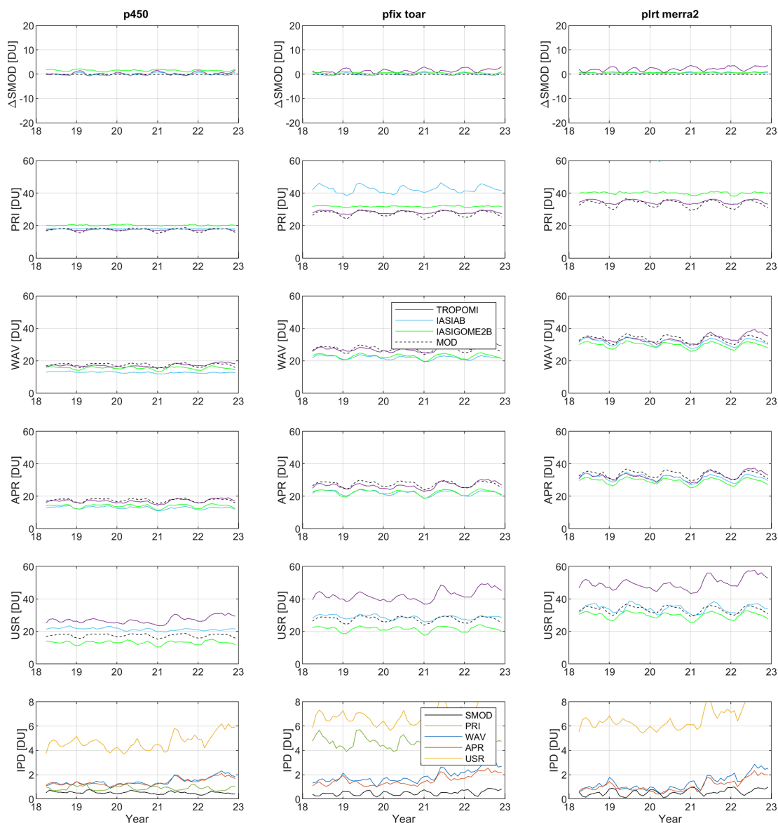
Figure 4. Same as Fig. 3 but for the overlapping period (May 2018–December 2022) of TROPOMI (purple), IASI-AB (blue), and IASI+GOME-2B (green), restricted to their common spatiotemporal sampling. Note that the IASI-AB PRI data is just above 60 DU for the lapse-rate tropopause definition (third column).
