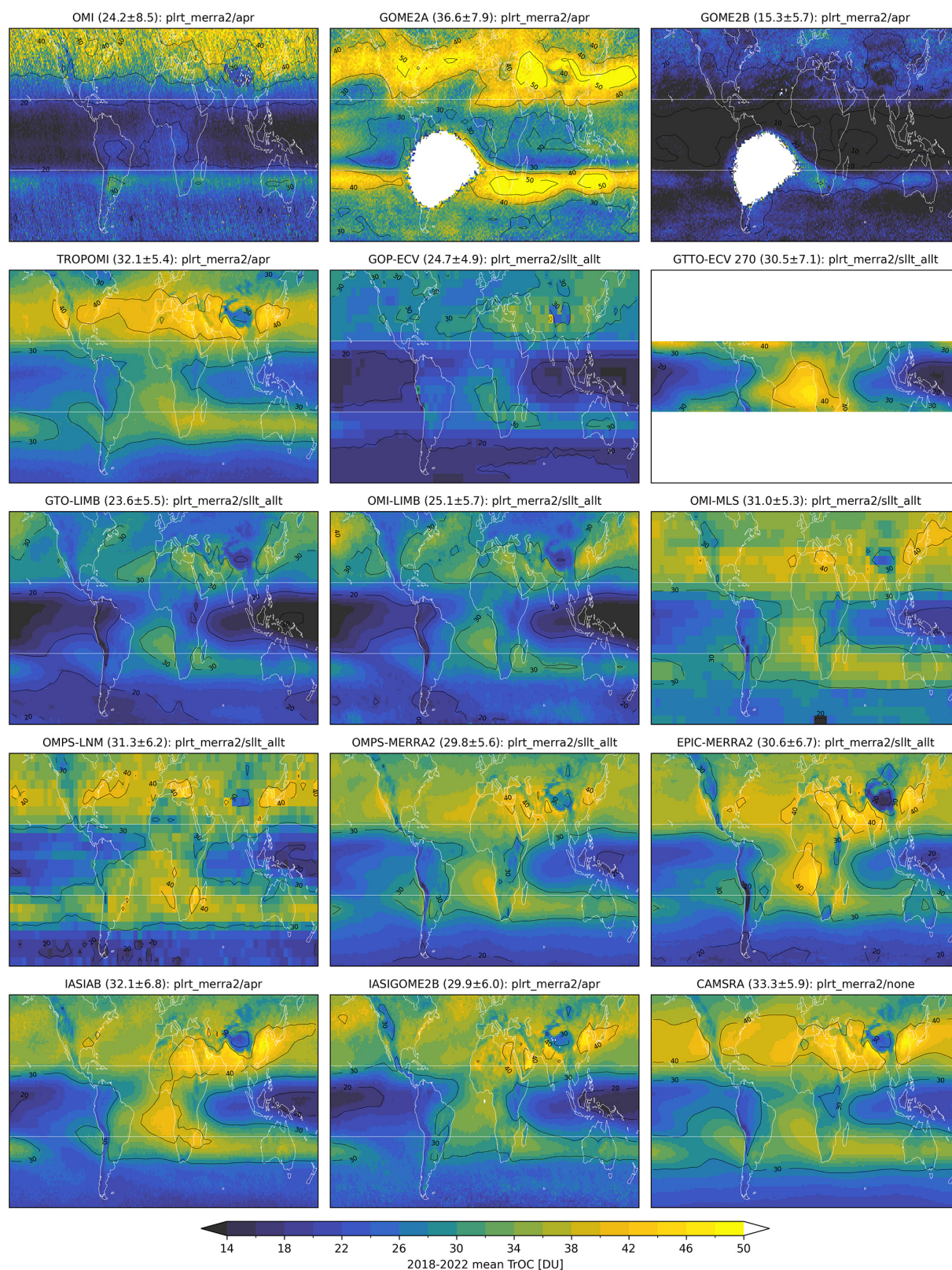
Figure 7. Multi-annual mean (2018–2022) tropospheric ozone column (TrOC) distribution of fourteen satellite data products and CAMSRA after harmonisation, using the APR method for the Level-2 profile products and the CAMSRA fill-in method for the column products. Area-weighted mean and standard deviation of the near-global tropospheric column (60° N–60° S) are given between brackets.
