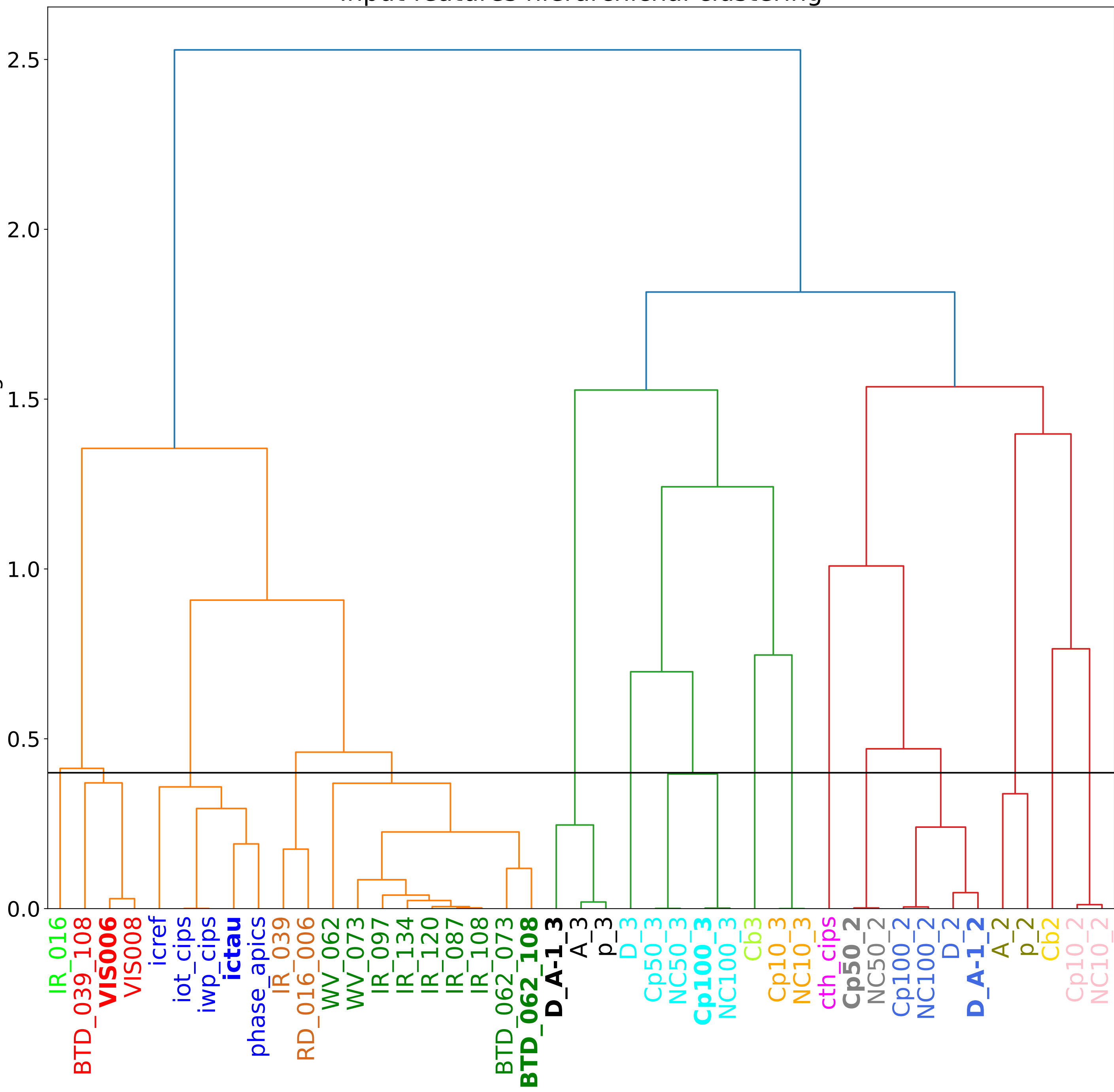
Input features hierarchichal clustering
