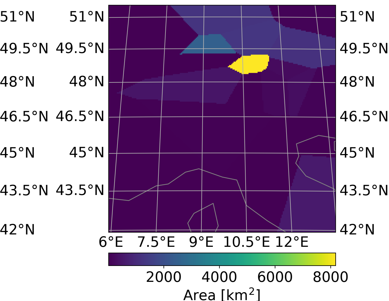
Area size closest convective cell
