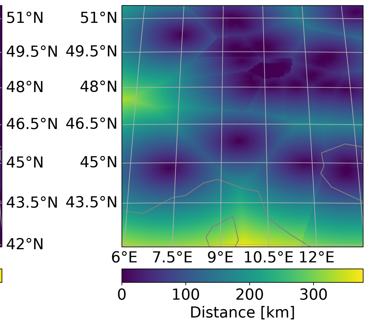
Distance to the closest convective cell
