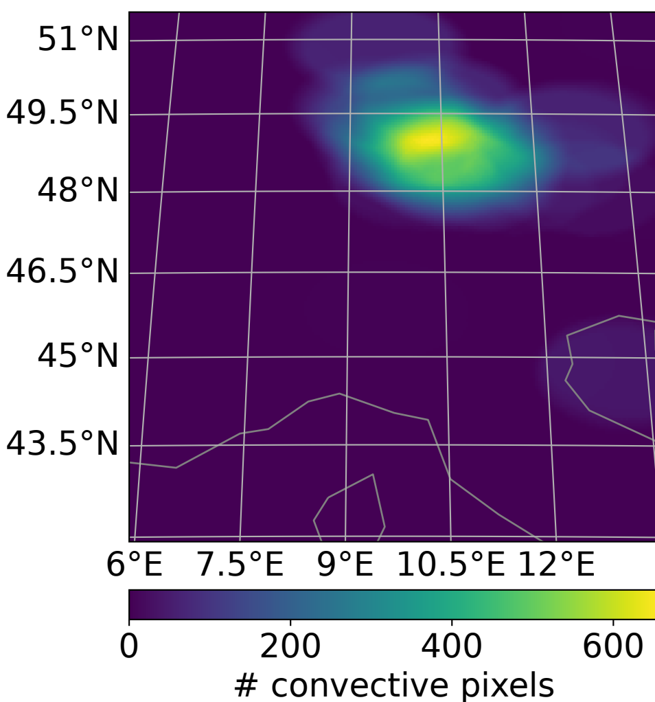
Convective pixels amount in surrounding radius of 100 km
