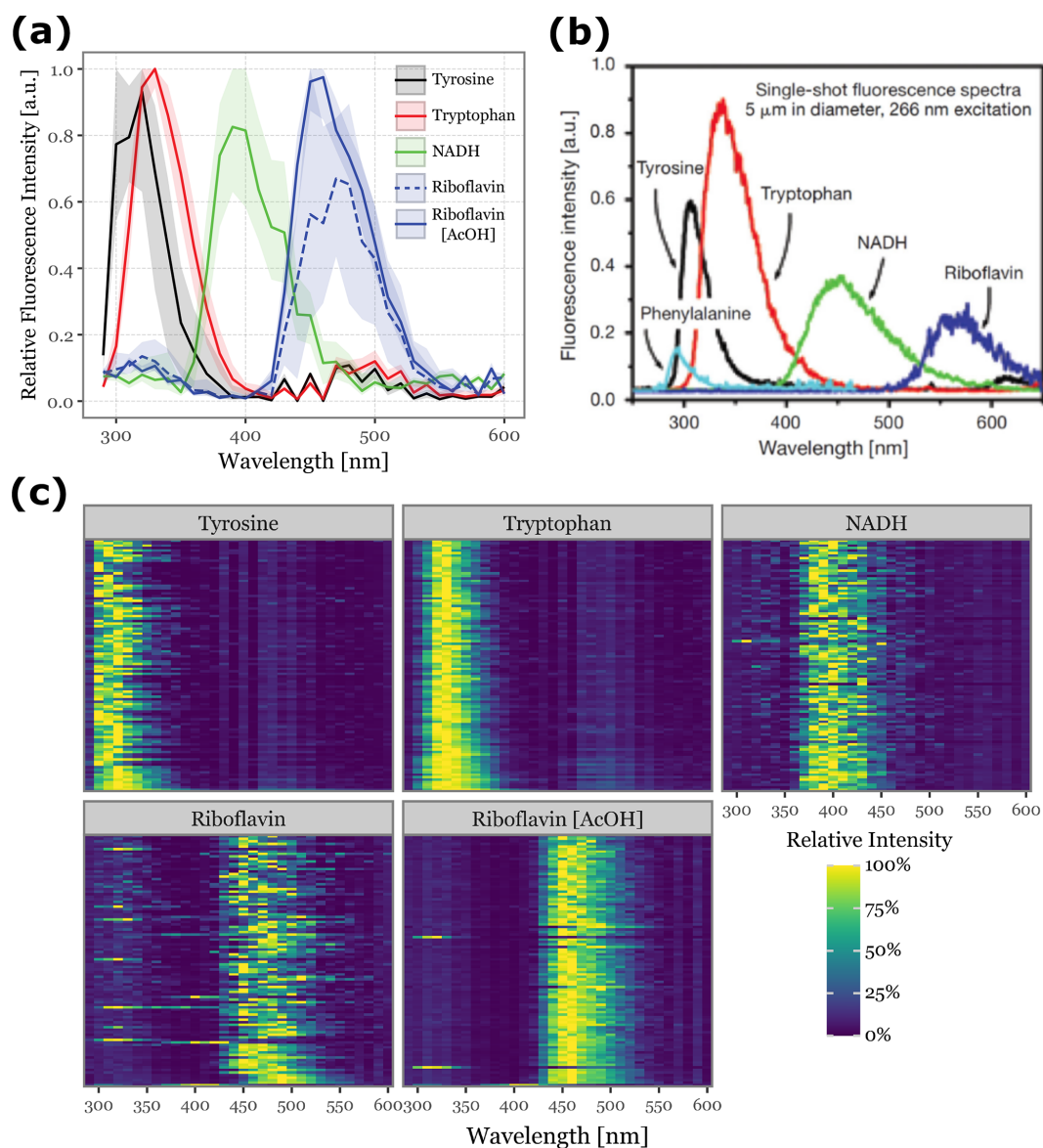
Figure 6. Fluorescence spectra detected for aerosolized biological fluorophores. Panel (a) shows the median fluorescence spectra, aggregated across all acquisitions, for the 100 most fluorescent particles during each fluorophore's sampling period. The shaded areas represent the interquartile range (25th to 75th percentiles). Panel (b) displays single-particle fluorescence spectra excited at 266 nm for common fluorophores found in biological particles, adapted from (Pan, 2015). The colors in Panels (a) and (b) are matched to facilitate comparison. Panel (c) presents a heatmap of the fluorescence spectra for the 100 most fluorescent particles from each fluorophore, ordered from top to bottom.
