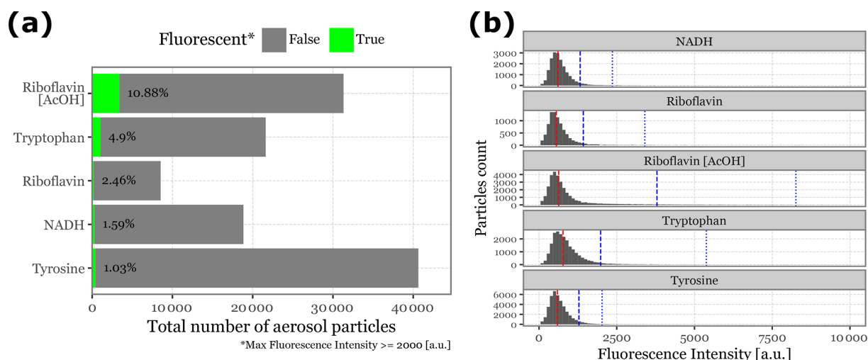
Figure 5. Particle count and fluorescence intensity distribution for biological fluorophores. Panel (a) displays a bar plot showing the total number of aerosol particles generated and detected by Rapid-E over a 10 min period. The green bars (and text) represent the fraction of particles detected as fluorescent, based on a threshold of 2000 a.u. for peak intensity at any given time or wavelength. Panel (b) presents histograms illustrating the intensity distribution of all detected particles during the aerosolization of each fluorophore. The red line indicates the median intensity for each group, while the blue dashed line and blue dotted line represent the 95th and 99th percentiles, respectively.
