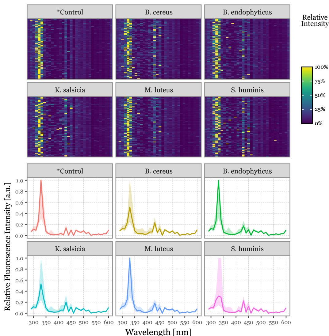
Figure 7. Fluorescence spectra for the aerosolized bacterial samples. In the top panel, heatmaps display the relative fluorescence intensity detected across all wavelengths within the detector's range for the top 100 most intensely fluorescent particles. The bottom panel shows the same data represented as line plots, with the solid line indicating the median value across all samples and the shaded area representing the interquartile range (25th to 75th percentiles).
