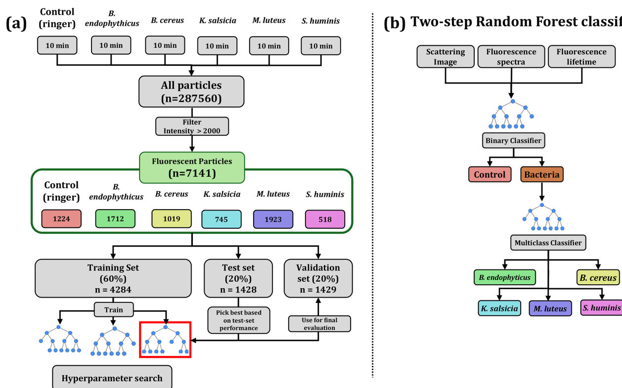
Figure 4. Data flow scheme and model hierarchy. Panel (a) illustrates how the experimental data is handled, filtered and used to train, evaluate and ultimately validate the models. Panel (b) visually describes the two-step approach employed for classifying aerosol particles using random forests: the first step involves a binary classifier to determine whether a particle is bacterial, and the second step employs a multiclass classifier to discriminate between bacterial species if the particle is identified as bacterial by the previous model.
