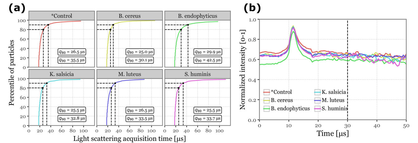
Figure 3. Light scattering intensity acquisition statistics. Panel (a) displays the cumulative distribution functions for the total time of light scattering acquisition per sample for each of the sample groups. Dashed lines and the text boxes indicate the values for the 80th and 90th percentiles. Panel (b) shows the median normalized intensity across all scattering angles as a function of acquisition time for each of the sample groups. The vertical dashed line marks the selected threshold of 30 \mu\text{s} .
