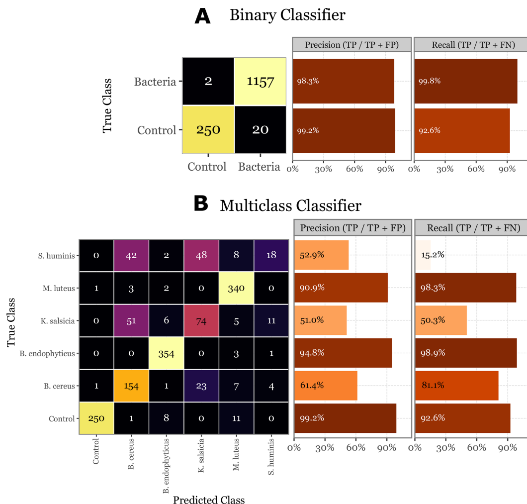
Figure 11. Evaluation of the skill of the Random Forest classifier on the validation set. On (a) the confusion matrix of the validation set for the binary classifier, with the class-specific precision and recall metrics on the right-side bar plots. On (b) the same but for the multi-class classifier. Control class added for comparison and to show the performance on the 20 control samples that the binary classifier predicted as bacteria.
