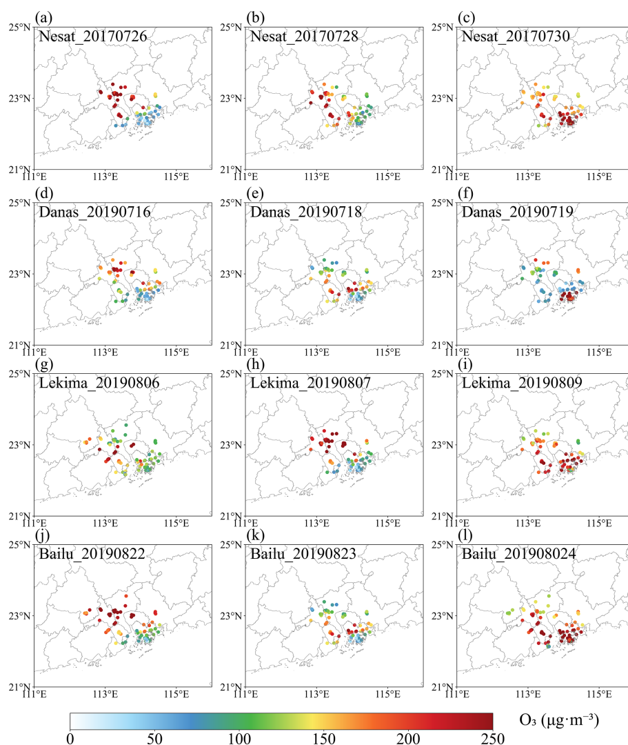
Figure 4. Spatial distribution of MDA8 O 3 surface concentrations in the GBA during (a–c) TC Nasat, (d–f) TC Danas, (g–i) TC Lekima and (j–l) TC Bailu.
