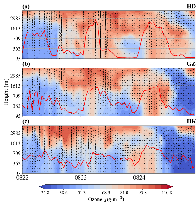
Figure 11. The figure displays time series of the simulated ozone and wind profile between 00:00 LT on 22 August and 00:00 LT on 25 August at three sites (Huadu, Guangzhou and Hong Kong). The vertical wind speed has been amplified by a factor of 10 to enhance clarity. In the figure, the red line indicates the height of the boundary layer.
