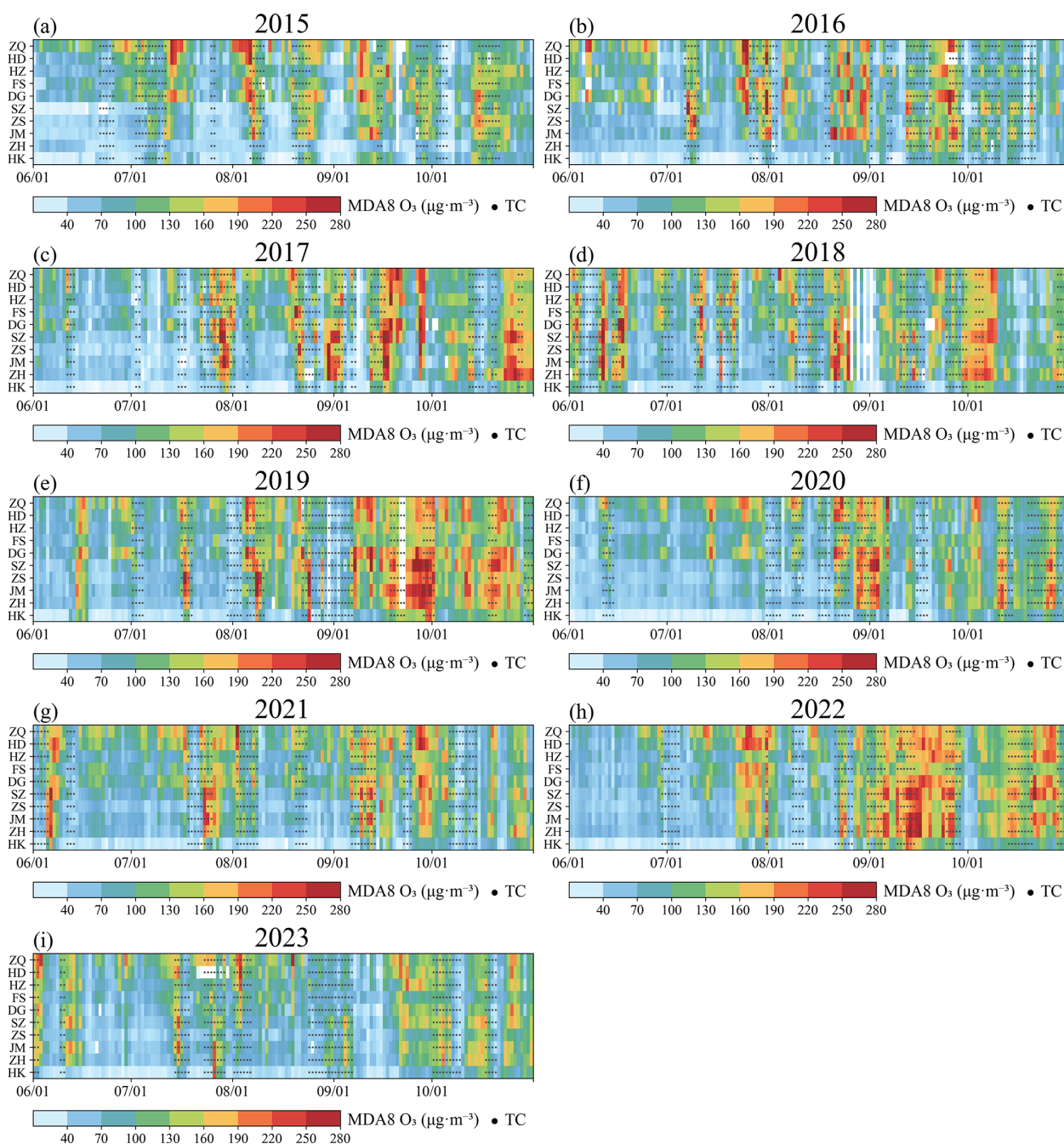
Figure 3. The maximum daily 8 h average (MDA8) \text{O}_3 in 10 cities in the GBA in (a) 2015, (b) 2016, (c) 2017, (d) 2018, (e) 2019, (f) 2020, (g) 2021, (h) 2022, and (i) 2023 from June to October. The national standard for ambient air quality for MDA8 \text{O}_3 is 160 \mu\text{g m}^{-3} in China. These cities are sorted by latitude. The black dots represent the days of TC, where the TC track enters ( 10\text{--}30^\circ \text{N} , 100\text{--}130^\circ \text{E} ).
