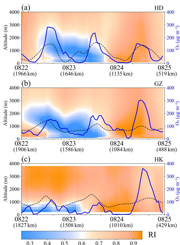
Figure 10. The recirculation index (shaded) was calculated using the wind profile radar at (a) the HD station, (b) the GZ station, and (c) the HK station from 22 to 25 August. Black dashed and blue lines represent the height of the boundary layer and the concentration of O_3 , respectively. The distance in brackets below the date on the x-axis represents the distance from TC Bailu to the wind profile radars at that moment.
