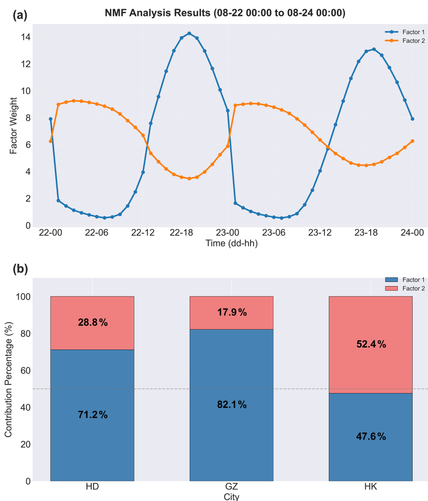
Figure 7. (a) Two factor time series (22–24 August). (b) Proportion of local generation and regional transmission in HD, GZ and HK.
