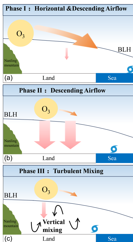
Figure 15. A schematic diagram illustrating the dynamic response of airflow and \text{O}_3 within the height of the boundary layer height (BLH) of the GBA to the approaching tropical cyclone (TC). (a) Phase I: Horizontal & Dwindraft Control – the pink arrows represent the dwindraft airflow from the periphery of the TC, the orange arrows indicate the northeasterly winds that transport \text{O}_3 horizontally across the GBA. (b) Phase II: Descending Airflow. (c) Phase III: Vertical Mixing – the black arrows depict the vertical mixing of air and \text{O}_3 within the boundary layer.
