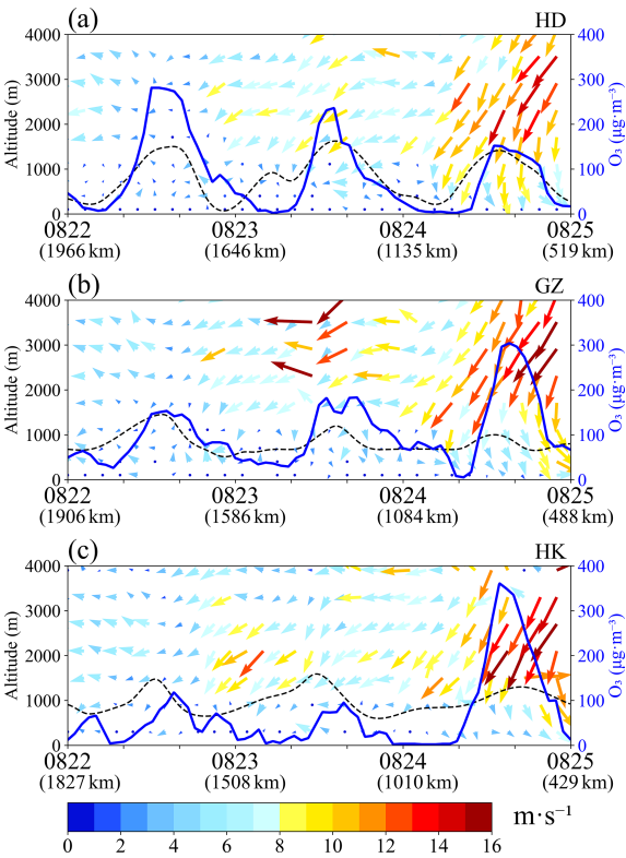
Figure 9. Horizontal wind (vector arrows) measured by wind profile radar at the (a) HD, (b) GZ, and (c) HK stations from 22 to 25 August. The black dashed and blue lines represent the height of the boundary layer and the concentration of O 3 , respectively. The distance in brackets below the date on the x-axis represents the distance from TC Bailu to the wind profile radars at that moment.
