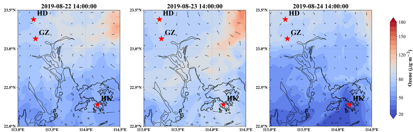
Figure 6. This figure illustrates the spatiotemporal distribution of ozone concentrations and wind fields simulated by WRF-Chem at different times within the Pearl River Delta region. The stars in the figure denote the locations of three radar stations.
