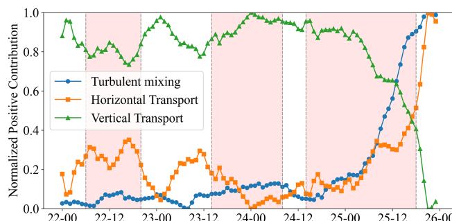
Figure 14. This normalized time series shows the contributions of three dynamical processes (horizontal transport, vertical transport, and turbulent mixing) to ozone pollution in the Pearl River Delta region. The dashed lines divide the processes into three distinct periods: a period dominated by horizontal and descending transport (Period I), a period with enhanced descending transport (Period II), and a period characterized by increased turbulent mixing (Period III).
