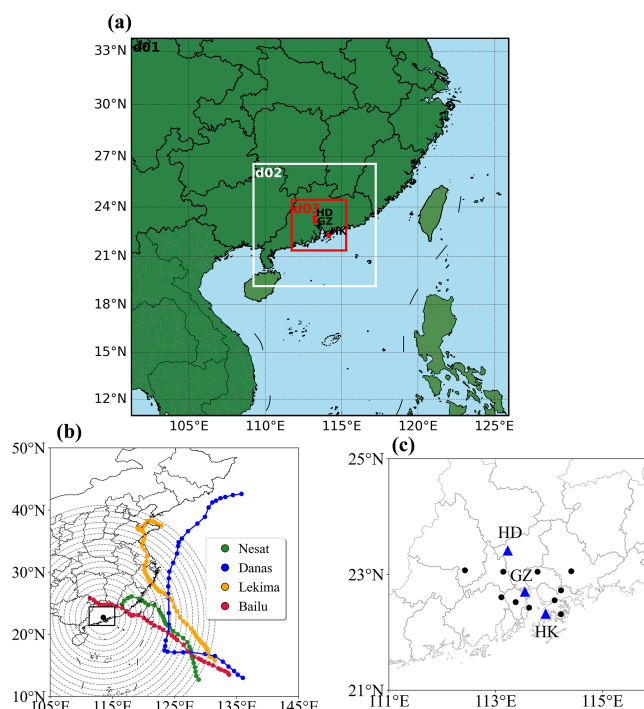
Figure 1. (a) the simulation domain is illustrated, with three monitoring sites annotated: Huadu ( 23.4^\circ\text{N} , 113.2^\circ\text{E} ), Guangzhou ( 22.7^\circ\text{N} , 113.5^\circ\text{E} ) and Hong Kong ( 22.3^\circ\text{N} , 114.2^\circ\text{E} ). These locations are strategically positioned to capture spatial variations within the study area. (b) Tropical Cyclone Nesat, Lekima, Danas, Bailu. The gray dashed circles are centered on the wind profiler radar in the middle of the GBA at GZ (black dot; 22.7^\circ\text{N} , 113.5^\circ\text{E} ), representing distances of 300–2000 km from the GBA, with intervals of 100 km between concentric circles. (c) Locations of the HD, GZ, and HK stations in the GBA. The black box indicates the location of the GBA. The black dots indicate the locations of the 10 cities shown in Fig. 3.
