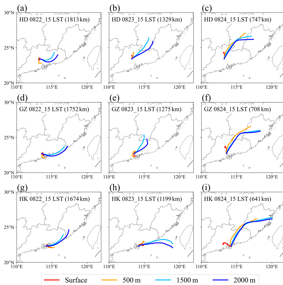
Figure 8. 24 h backward trajectories of (a–c) HD station, (d–f) GZ station, and (g–i) HK station at different vertical heights. (Heights of 0, 500, 1500, and 2000 m represent the surface, the middle of the boundary layer, the top of the boundary layer, and above the boundary layer, respectively. The distance in the character brackets on the top left of the subplot indicated the distance from TC Bailu to the wind profile radars at that moment.)
