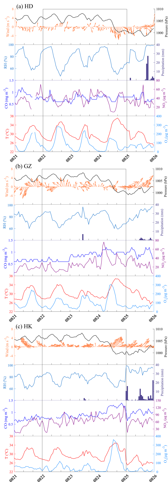
Figure 5. Time series of wind, air pressure, relative humidity (RH), 24 h precipitation, CO, NO 2 , temperature of 2 m ( T ), and O 3 at (a) HD, (b) GZ, and (c) HK stations from 21 to 25 August 2019. The black boxes indicate the study period.
