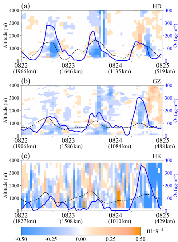
Figure 12. Vertical wind speed (color filled) was measured by wind profile radar at the (a) HD, (b) GZ, and (c) HK stations from 22 to 25 August. The black dashed and blue lines represent the height of the boundary layer and the concentration of O_3 , respectively. The distance in brackets below the date on the x -axis represents the distance from TC Bailu to the wind profile radars at that time.
