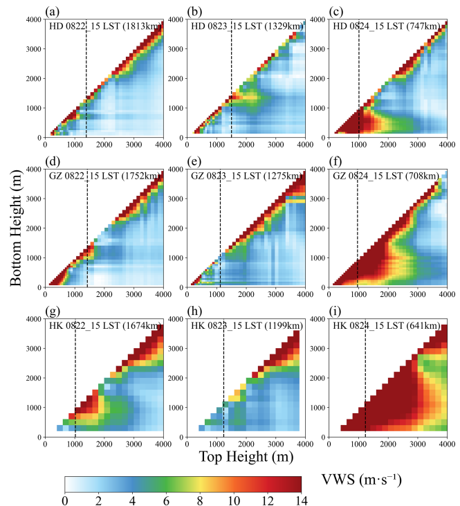
Figure 13. Vertical Wind Shear (VWS) from 22 to 24 August at (a–c) HD station, (d–f) GZ station, and (g–i) HK station. The black dashed line represents the height of the boundary layer. The distance in character brackets at the top left of the subplot indicated the distance from TC Bailu to the wind profile radars at that moment.
