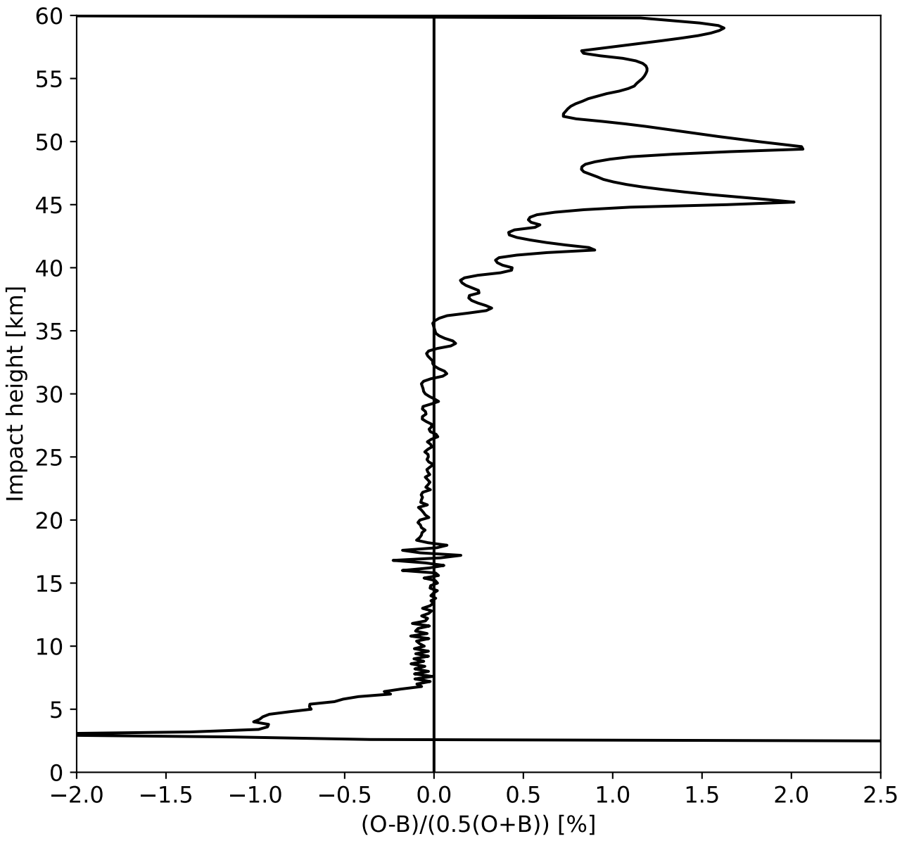
BA Global O-B statistics for all satellites provided by multiple centres
