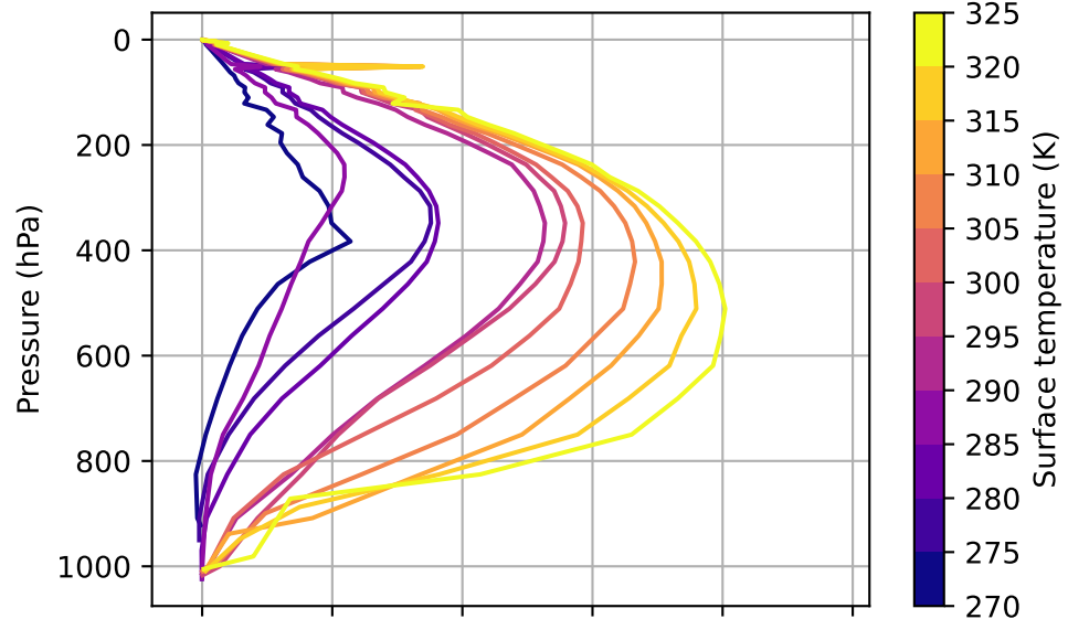
AIRS
