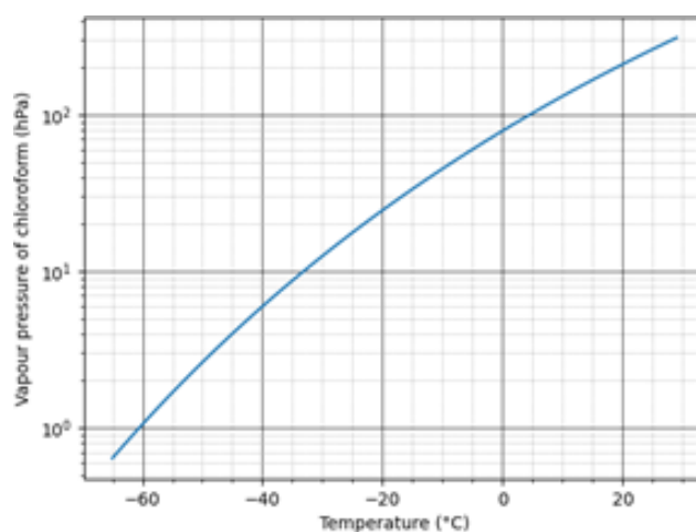
Figure 1. Vapour pressure of chloroform (hPa) vs. temperature ( ^\circ\text{C} ) adapted from Linstrom and Mallard (2026).
