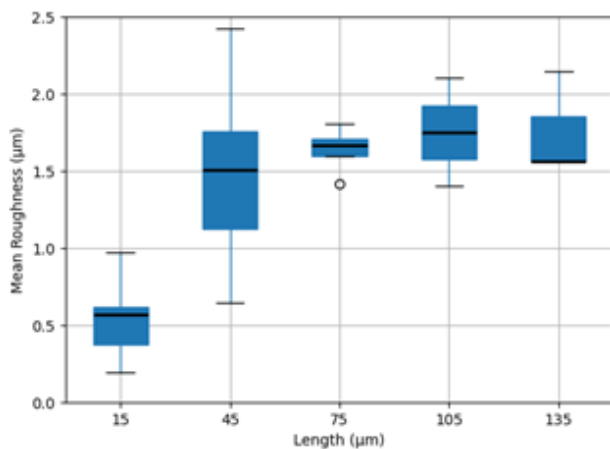
Figure 9. Statistical comparison of length ( \mu\text{m} ) vs. mean-roughness values ( \mu\text{m} ) across multiple selected areas of multiple ice crystals' surfaces ( n = 7 for each size bin). Circle indicates outlier.
