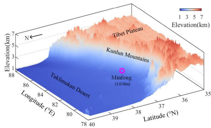
Figure S1. The Digital elevation map of the study site Mingfeng. Sloping terrain facilitates the upslope transport of dust along mountain ranges.
