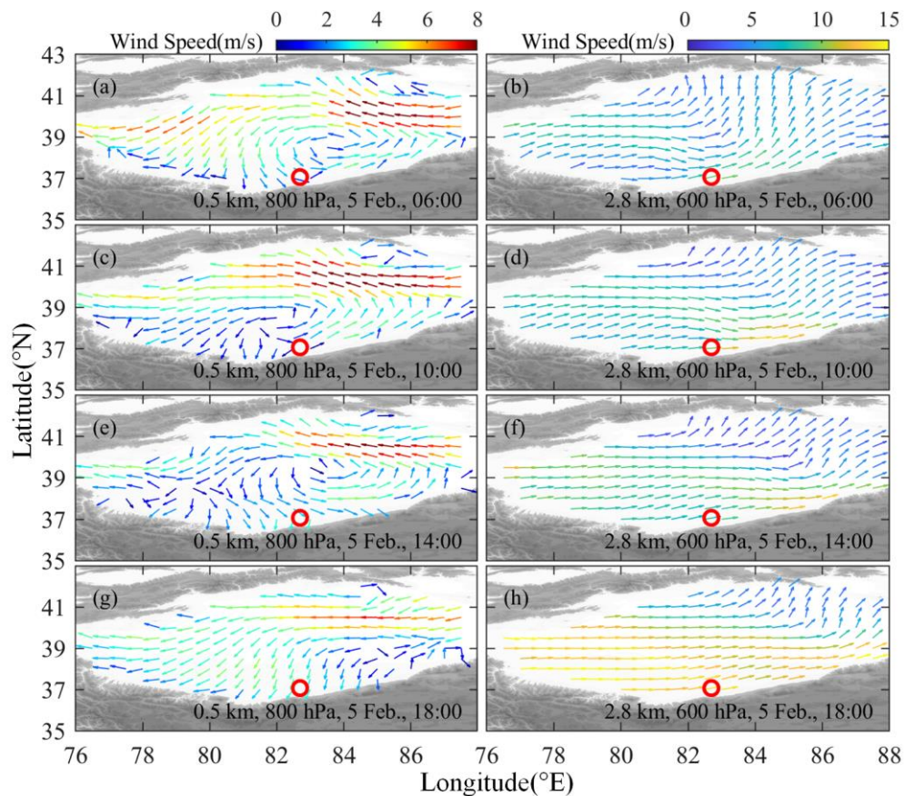
Figure S3. Wind vectors at 800 hPa (left) and 600 hPa (right) over the Taklimakan Desert from 6:00 to 18:00 LT (UTC+8) on 5 February 2022. The gray areas are the higher mountains, the white areas are the lower basin, and the red circle symbol is the study site. The life cycle of ice crystal cloud for (a-d) Stage-1 and (e-h) Stage-2 is shown.
